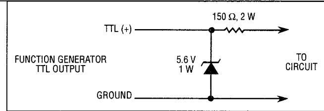
Figure 5. Circuit for Protection of TTL Output.
