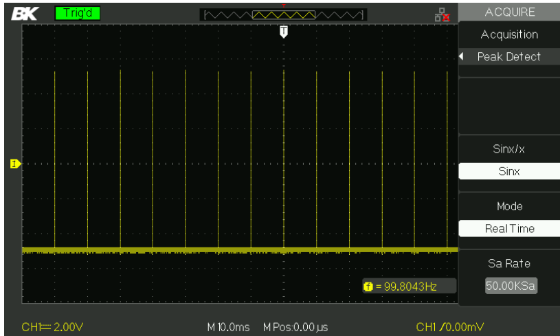
Figure 3.31 – Peak Detect
