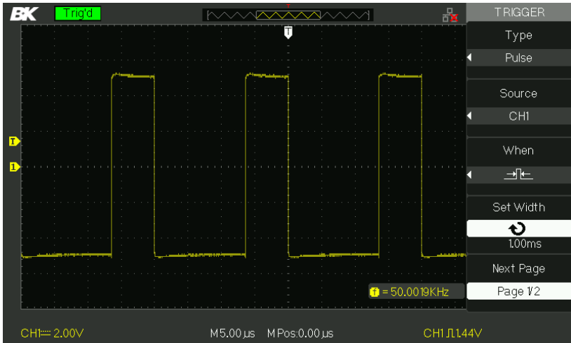
Figure 3.22 – Pulse Trigger Menu 1
