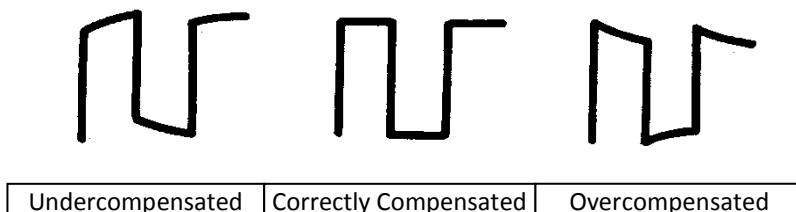
Figure 2.7 – Compensation Illustration
