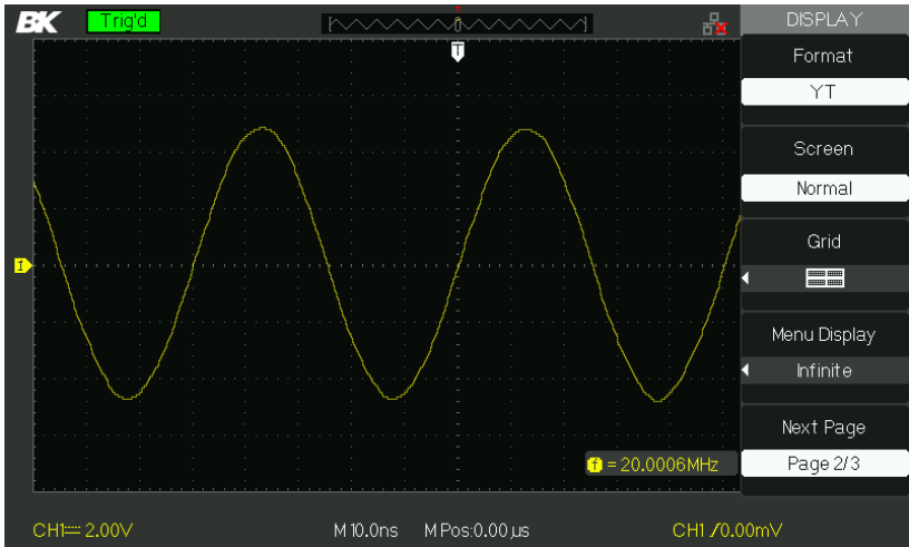
Figure 3.35 – Display Menu 2
