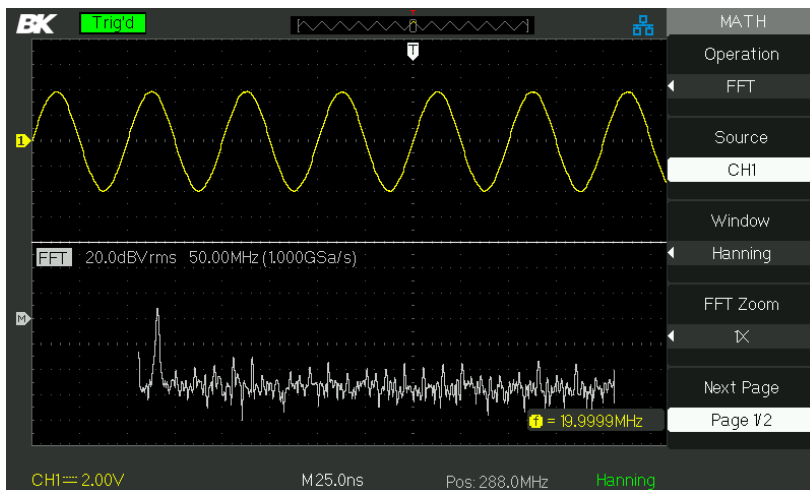
Figure 3.14 – FFT Function
