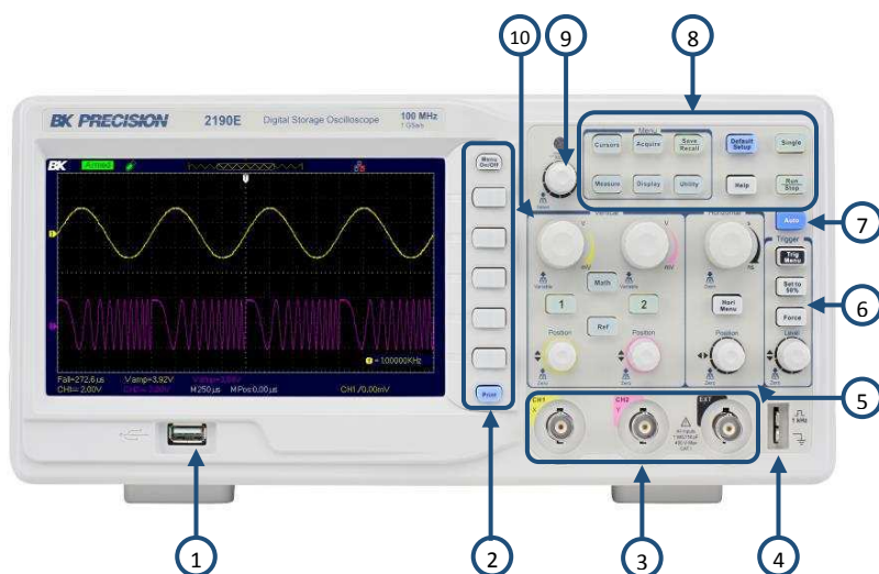
Figure 1.1 – Front Panel
