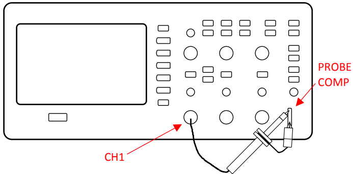
Figure 2.3 – Probe Compensation
