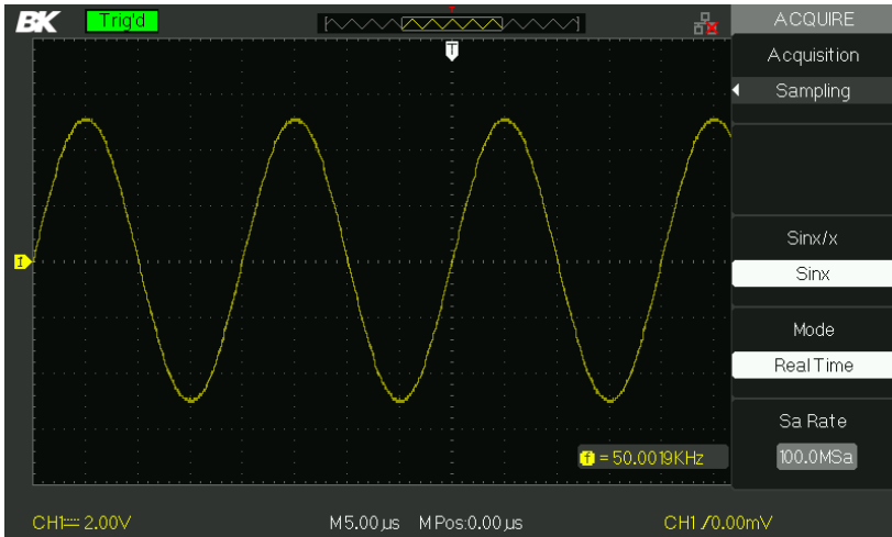
Figure 3.30 – Acquire Menu
