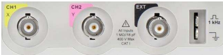
Figure 3.2 – Connectors
