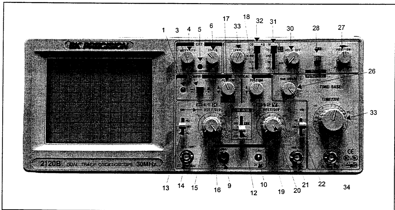
Fig. 2. Model 2120B Controls and Indicators.
