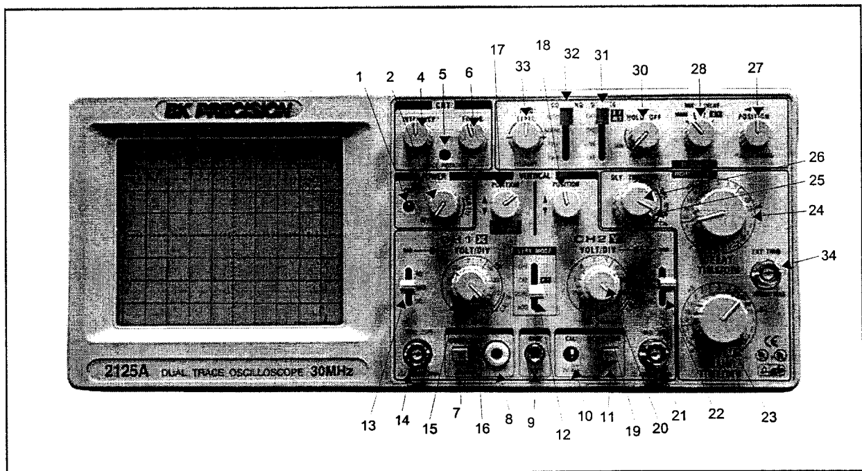
Fig. 1. Model 2125A Controls and Indicators.
