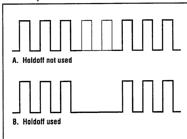
Fig. 4. Use of HOLDOFF Control.
