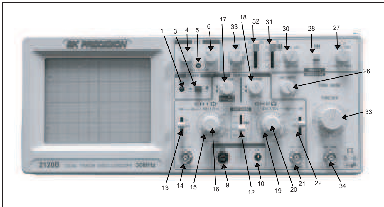
Fig. 2. Model 2120B Controls and Indicators.
