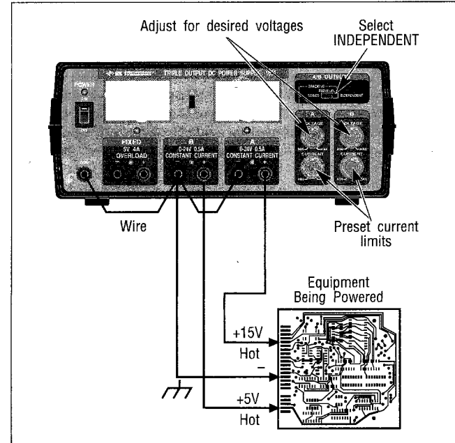
Figure 12. Typical hook-up using two differing positive voltages and a common negative.
