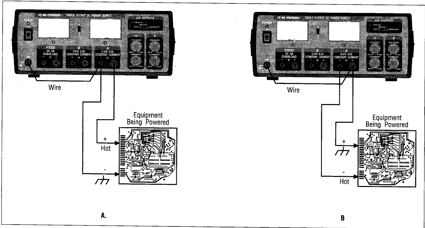
Figure 3. Independent operation grounding possibilities (sheet 1 of 2).
