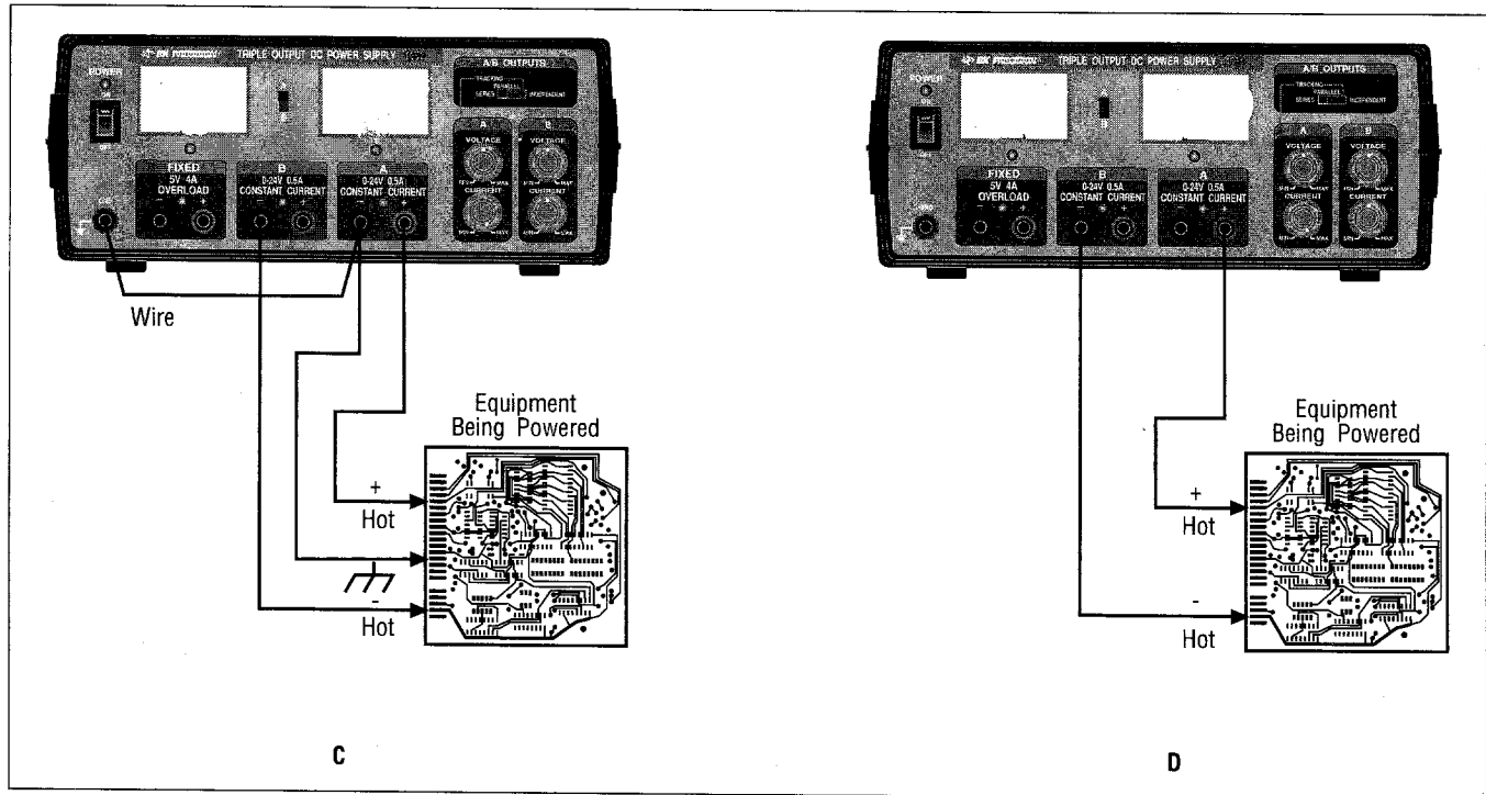
Figure 8. Series tracking (0-to-48 V) operation grounding possibilities (sheet 2 of 3).
