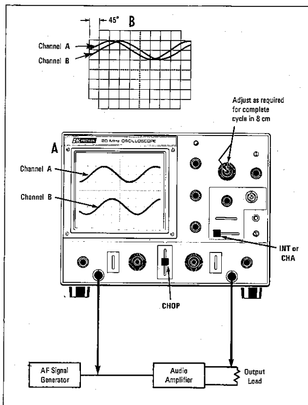
Fig. 24. Measuring amplifier phase shift.
