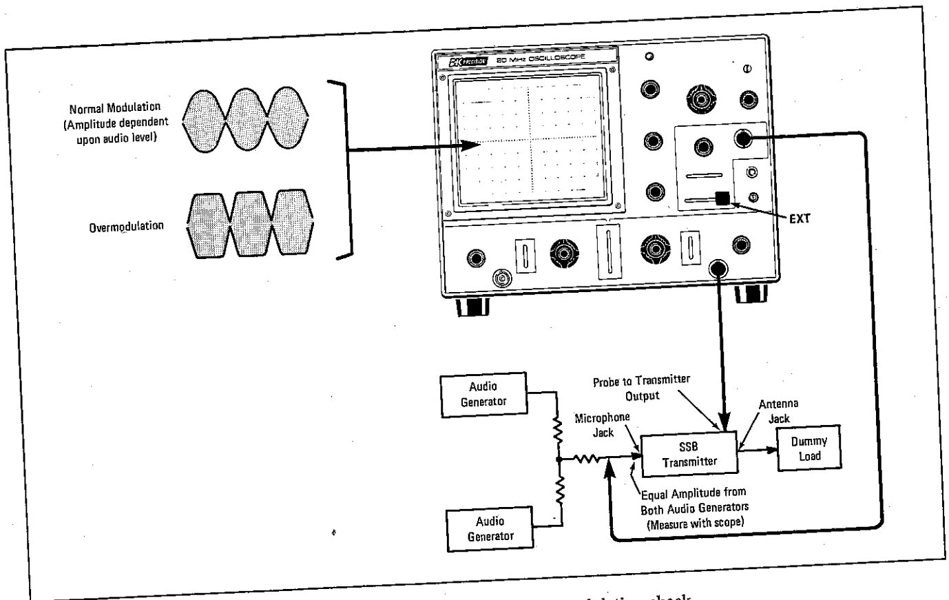
Fig. 23. Typical test set-up for SSB modulation check.
