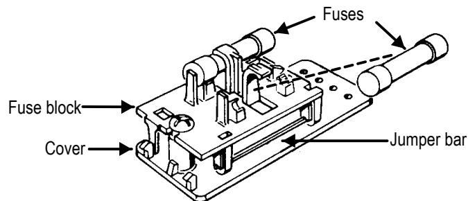
Figure 3-4. European fusing arrangement
