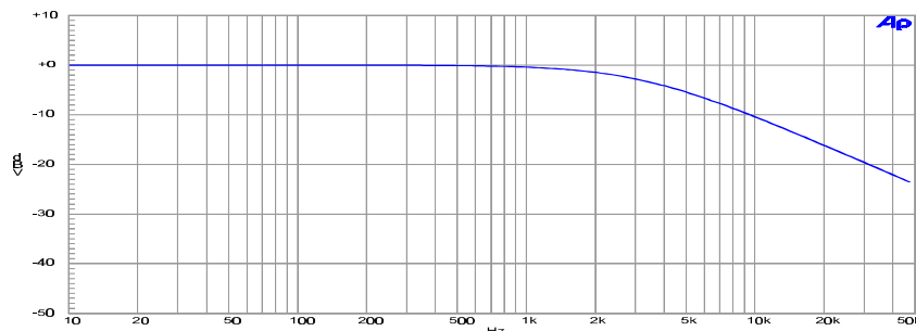
Figure 2-23. FIL-D50 50 \mu s De-emphasis Filter
