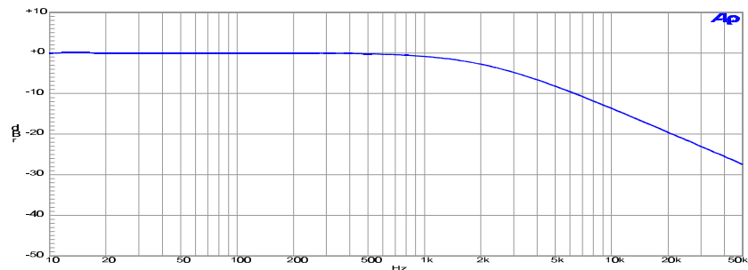
Figure 2-22. FIL-D75 75 \mu s De-emphasis Filter
