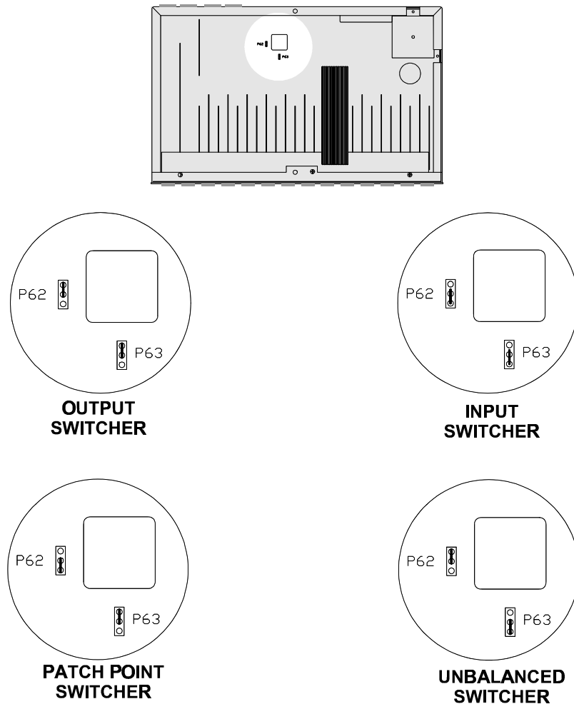
Figure 3-12. Switcher mode jumper positions
