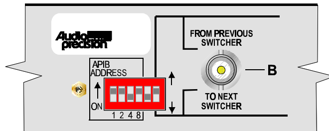
Figure 3-11. Unbalanced switcher address/mode switch
