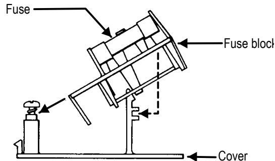
Figure 3-5. Changing fuse types
