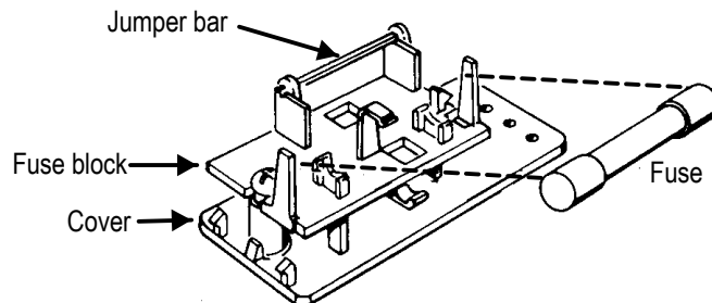
Figure 3-3. North American fusing arrangement
