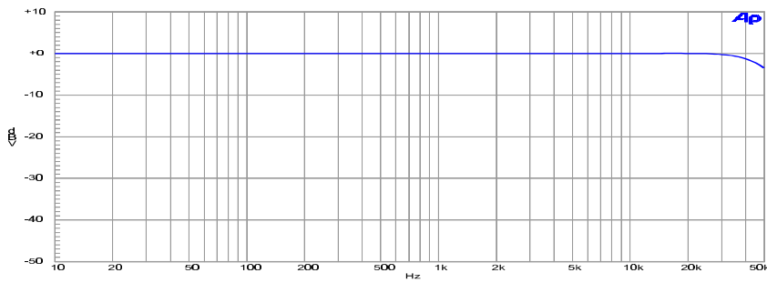
Figure 2-11. FLP-50K 50 kHz 3-pole Butterworth Low Pass Filter
