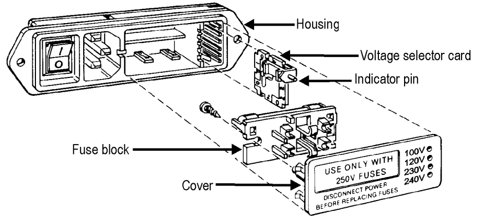
Figure 3-1. Changing power line voltage
