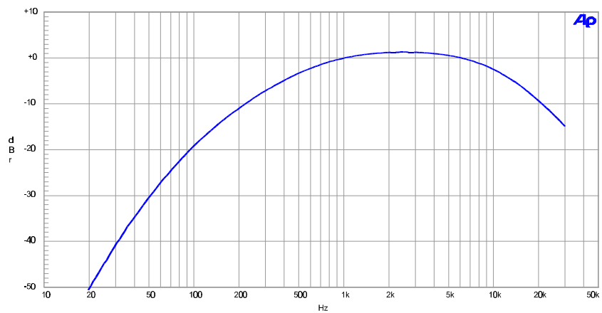
Figure 2-4. FIL-AWT ANSI-IEC “A” Weighting Filter
