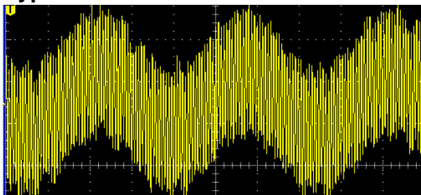
An oscilloscope capture of a switching amplifier output signal. The high-frequency, high-level switching carrier is shown riding the lower-frequency audio.
