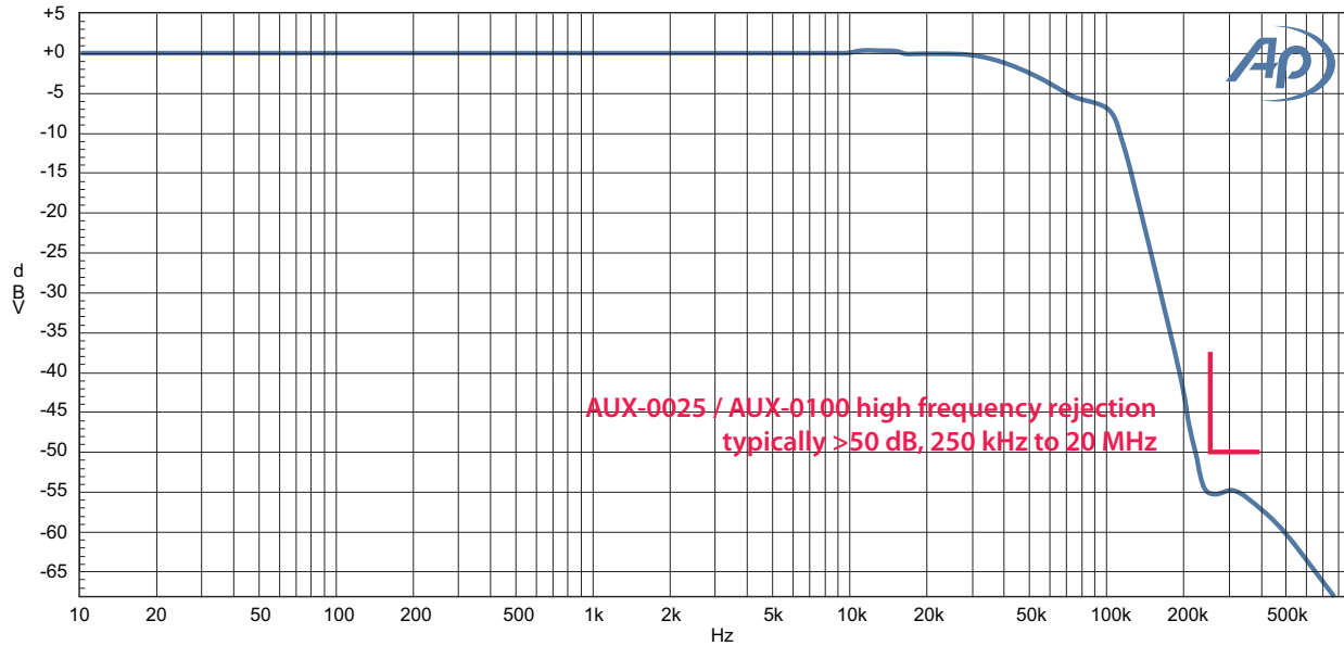
AUX-0025 and AUX-0100 filter cutoff
