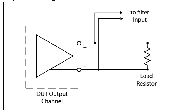
Connection detail, DUT output, AUX filter input and load resistor.
