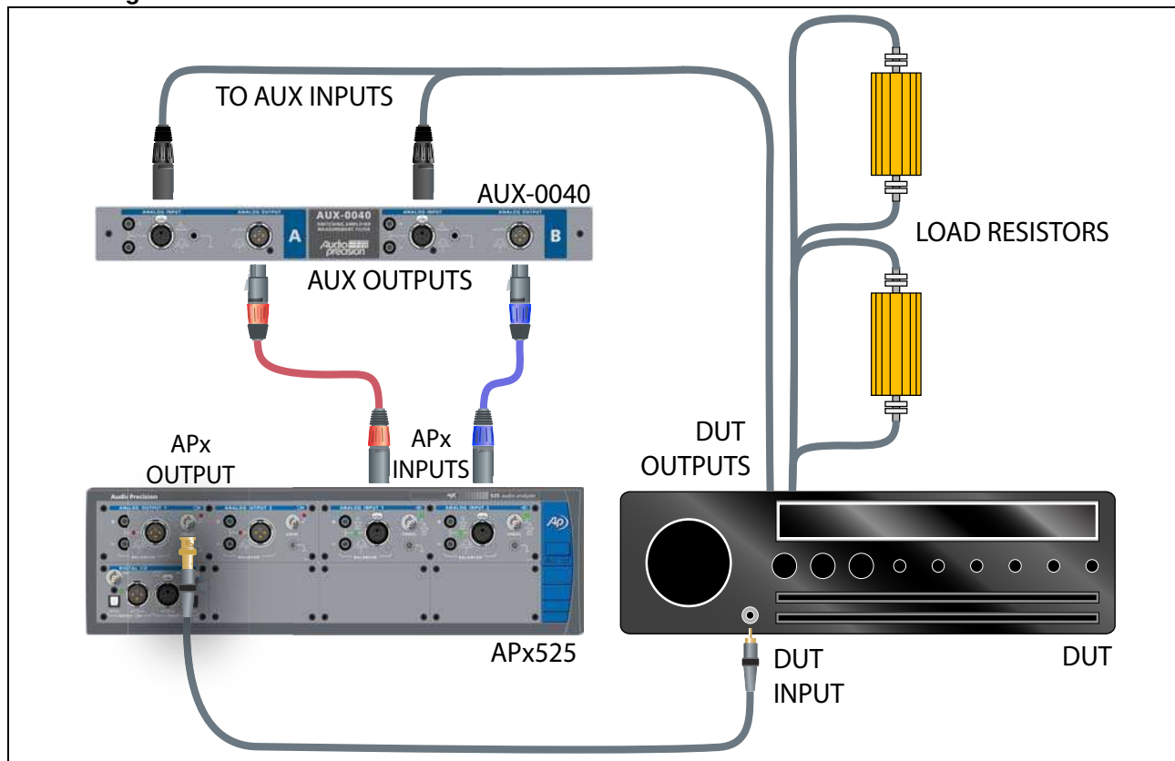
Diagram representing a switching amplifier whose outputs are connected to both the AUX-0025/AUX-0040 and to load resistors.
