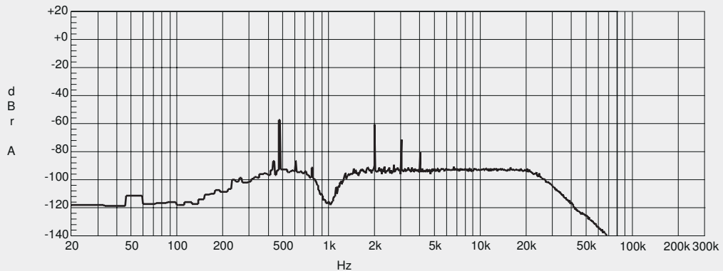
Figure 4-14. Spectrum with 22 kHz lowpass filter added
