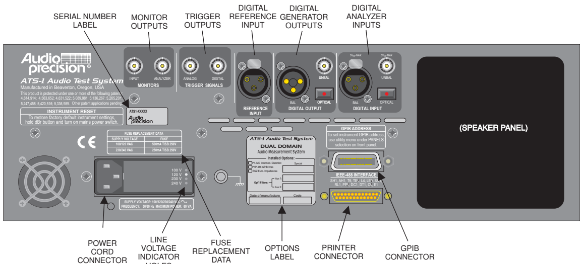
Figure 3-15. Rear panel overview
