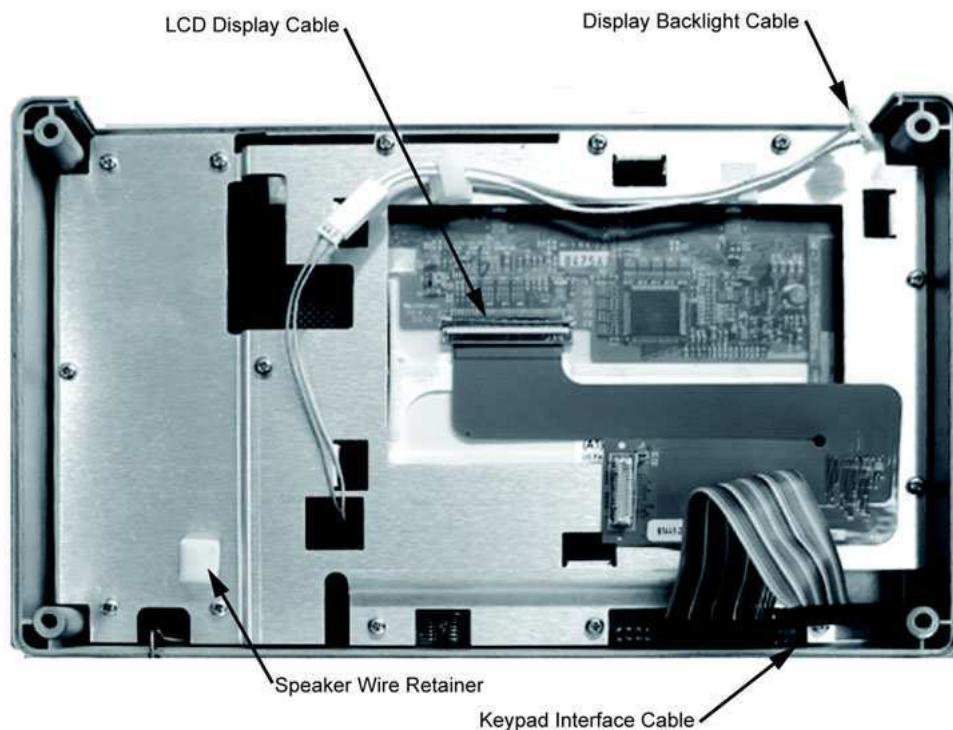
Figure 3-5. Front Panel Backing Plate
