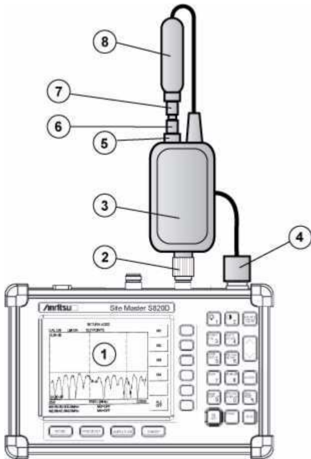
Figure 2-10. Two-Port Cable Loss Measurement Accuracy Connections
