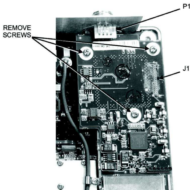
Figure 3-8. RF Detector PCB Replacement
