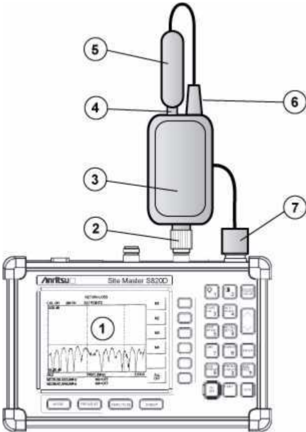
Figure 2-7. Two-Port Cable Loss General Connections
