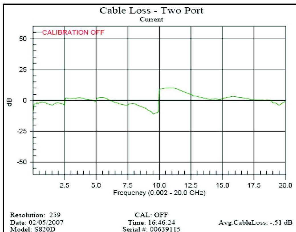
Figure 2-8. Cable Loss Two-Port Typical Waveform
