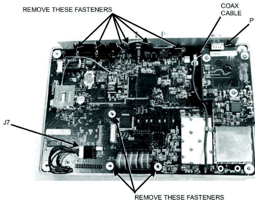
Figure 3-10. Main/RF PCB Assembly
