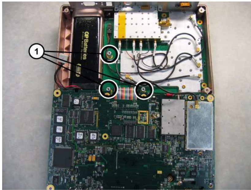
Figure 3-11. Main/RF PCB Removal
