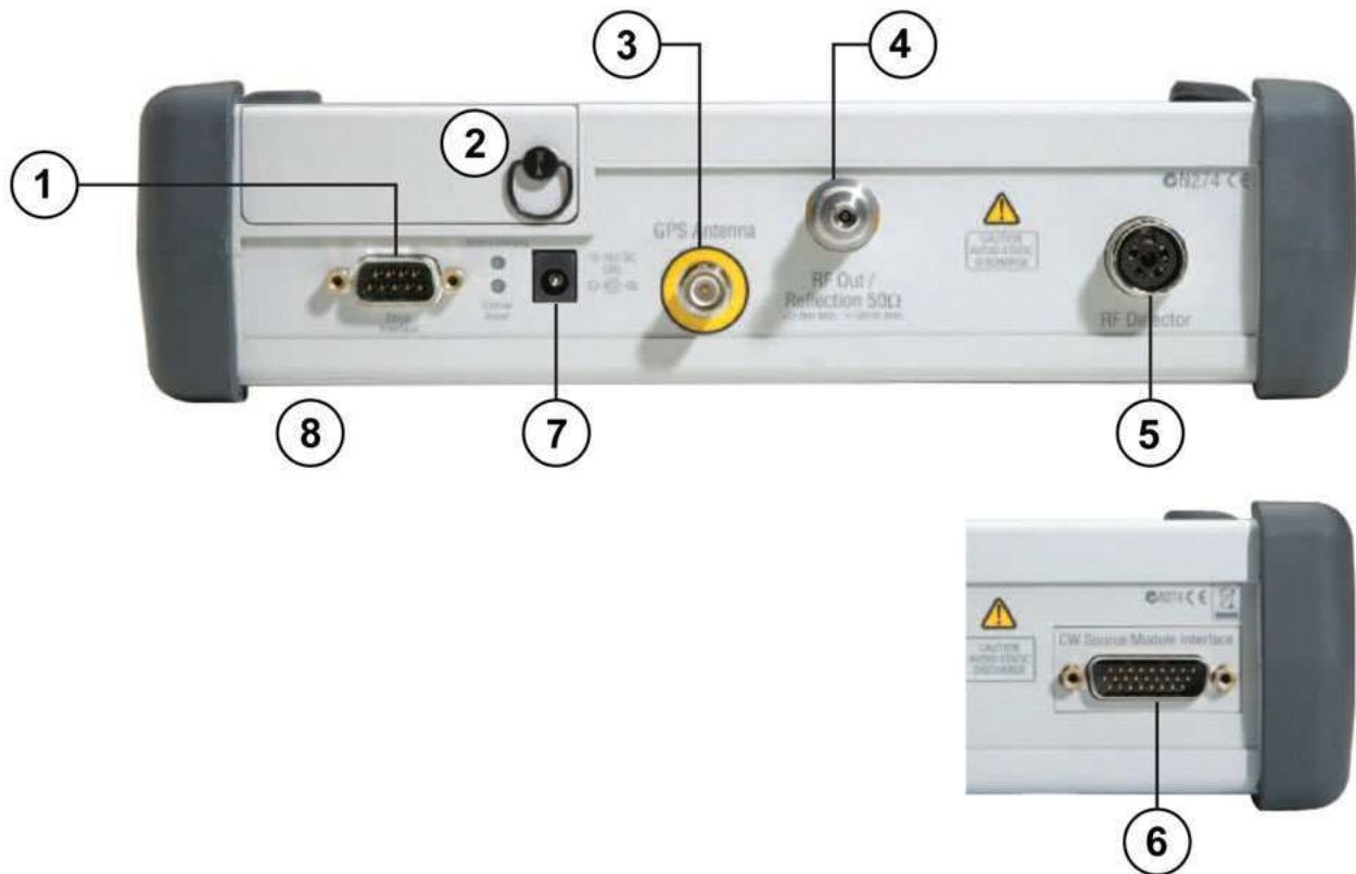
Figure 1-2. S810D/S820D Top Connectors with RF Detector Option on Right
