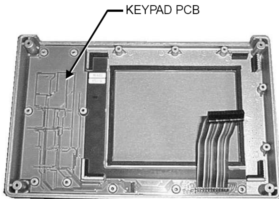
Figure 3-6. Front Panel Keypad PCB Location
