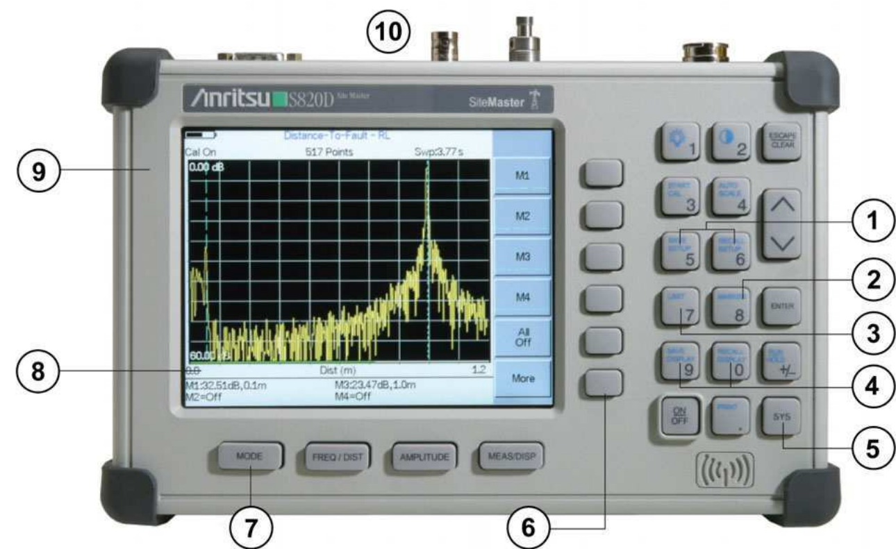
Figure 1-1. S810D/S820D Site Master Front Panel Hard and Soft Keys
