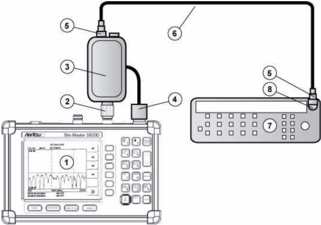
Figure 2-9. Two-Port CW Frequency Verification Connections
