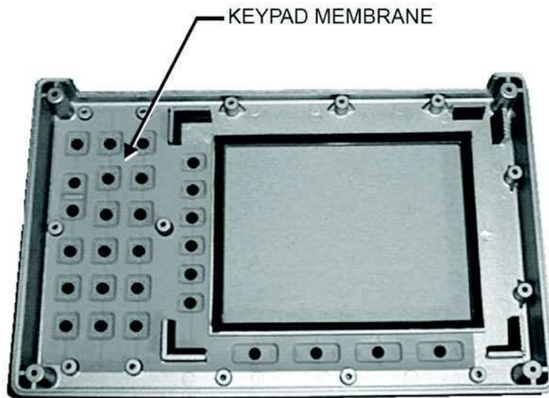
Figure 3-7. Front Panel Keypad Membrane
