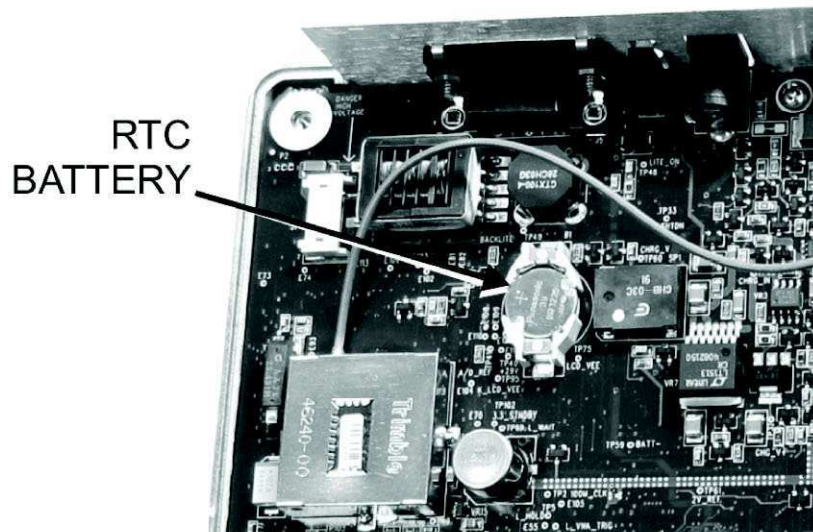
Figure 3-9. Real Time Clock Battery
