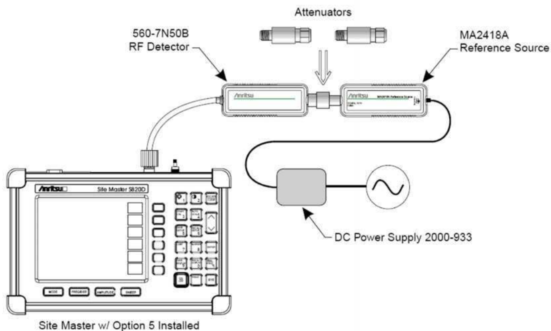
Figure 2-5. Power Monitor Verification Setup
