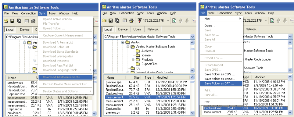
Figure 3-9. MST Dialog
