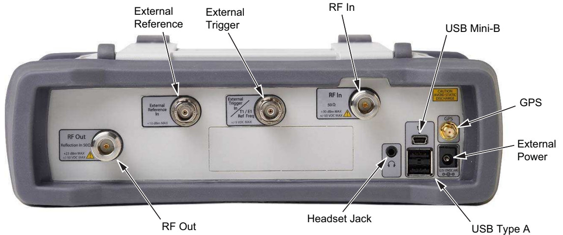
Figure 2-8. S332E Test Panel Connector
