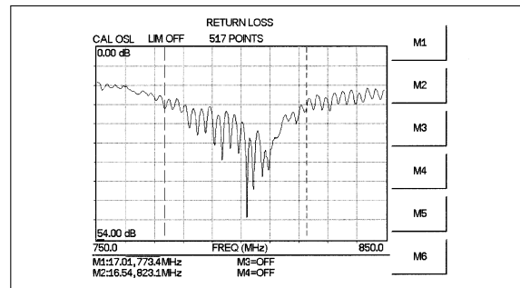
Return loss
