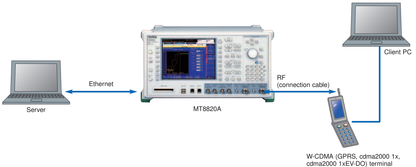
Sample MT8820A connection
