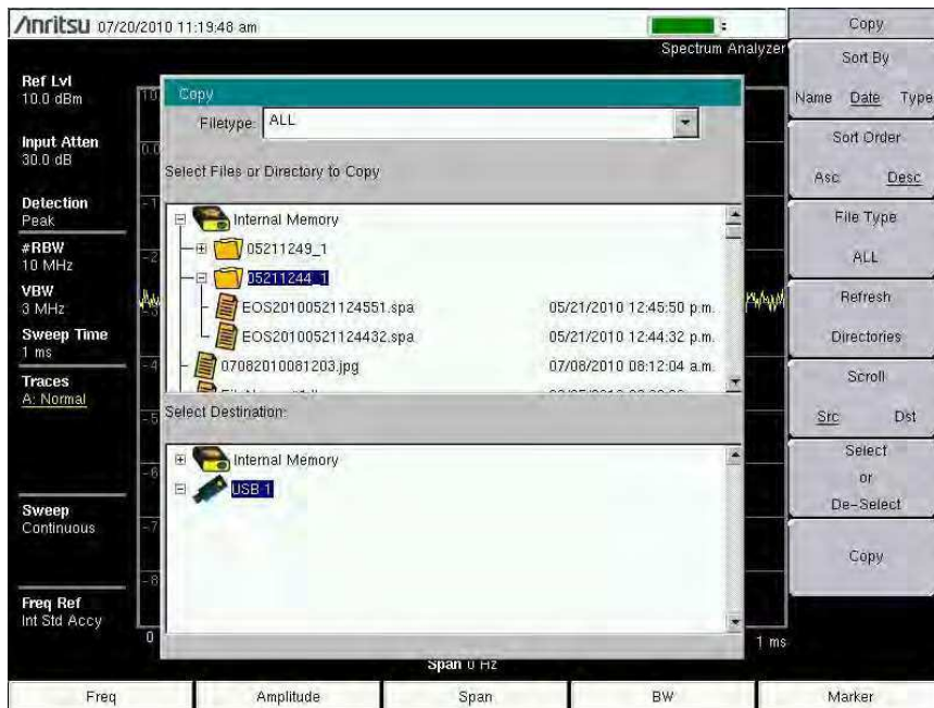
Figure 4-3. Expanded Folder
