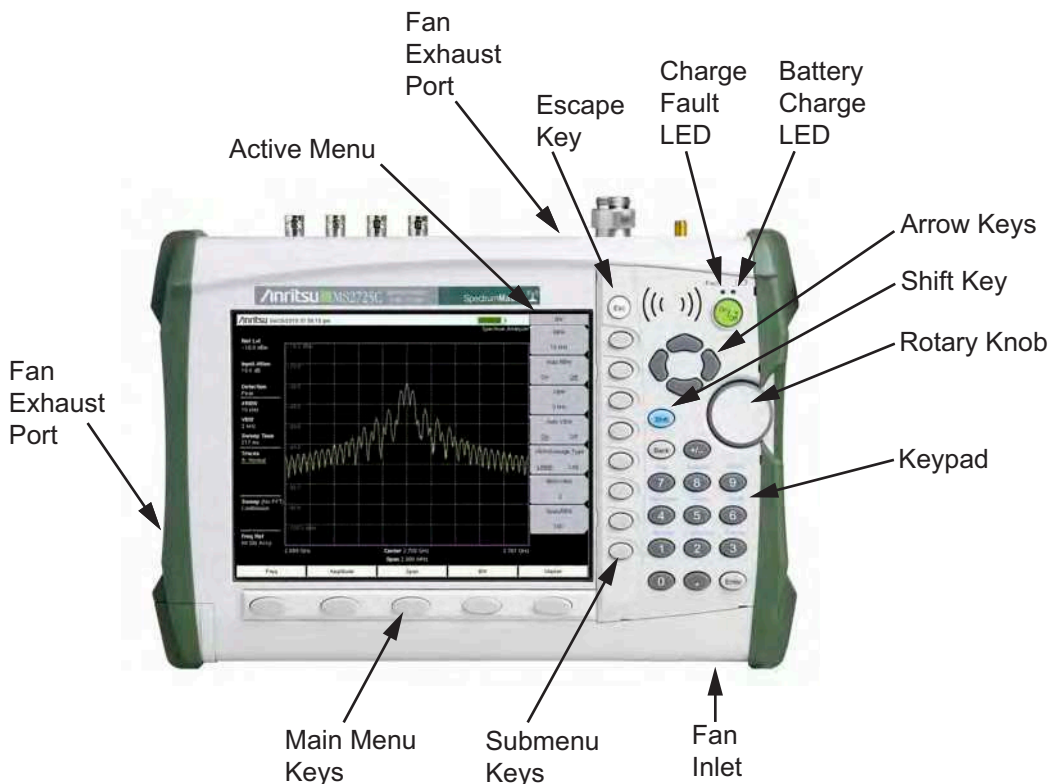
Figure 2-2. Front Panel Overview
