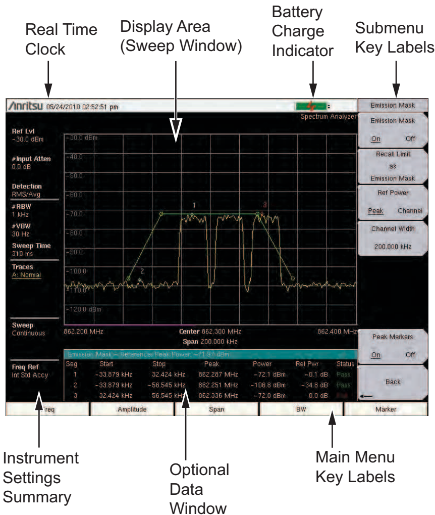
Figure 2-6. Spectrum Analyzer Display
