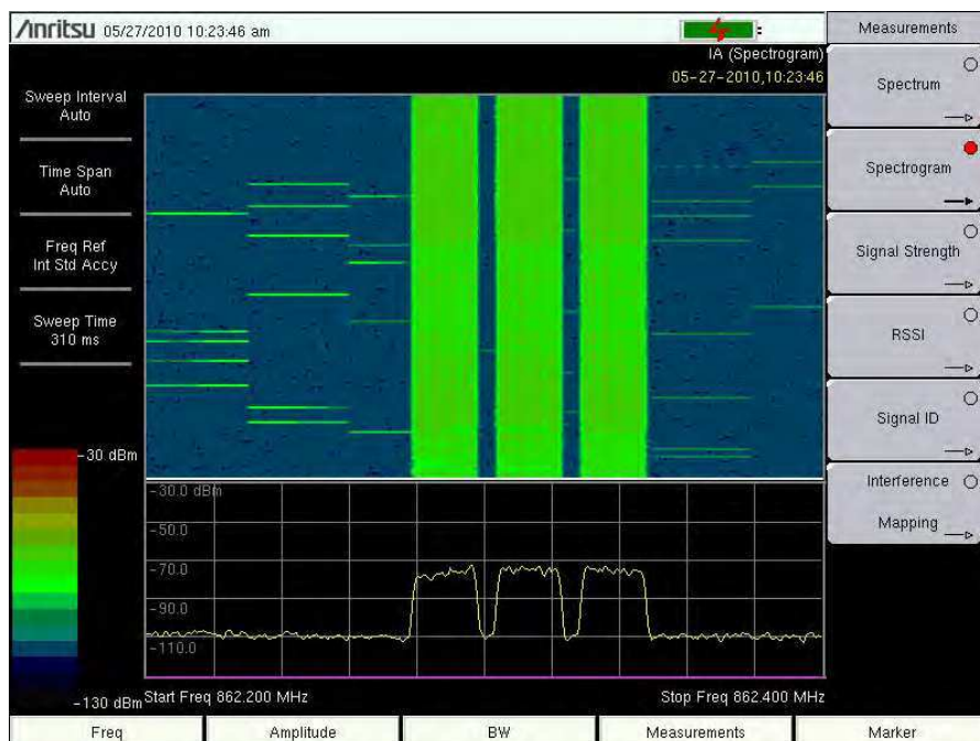
Figure 3-1. Spectrogram Example
