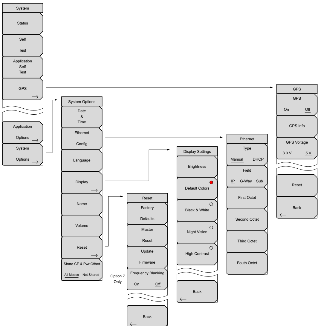
Figure 5-1. System Menu Map
