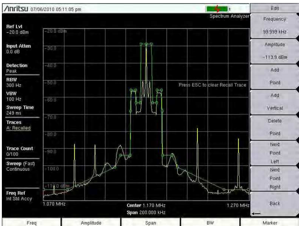
Figure 3-2. Complex Limit Line Example
