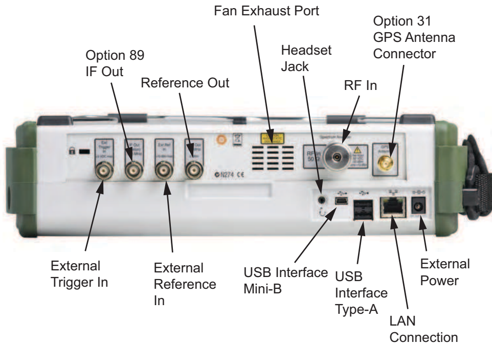
Figure 2-10. Test Panel Connectors for MS272xC
