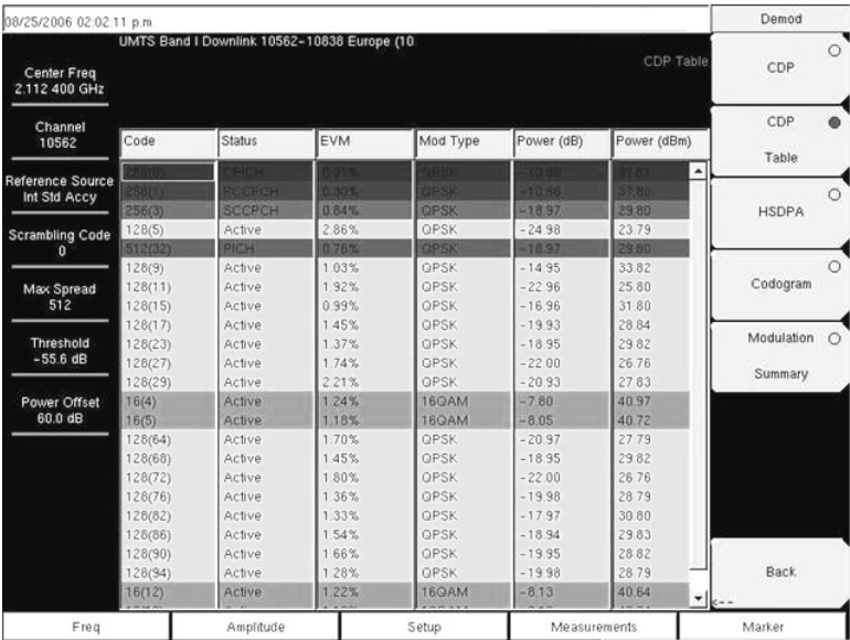
Figure 7-16. Code Domain Power Table Measurement Screen Example
