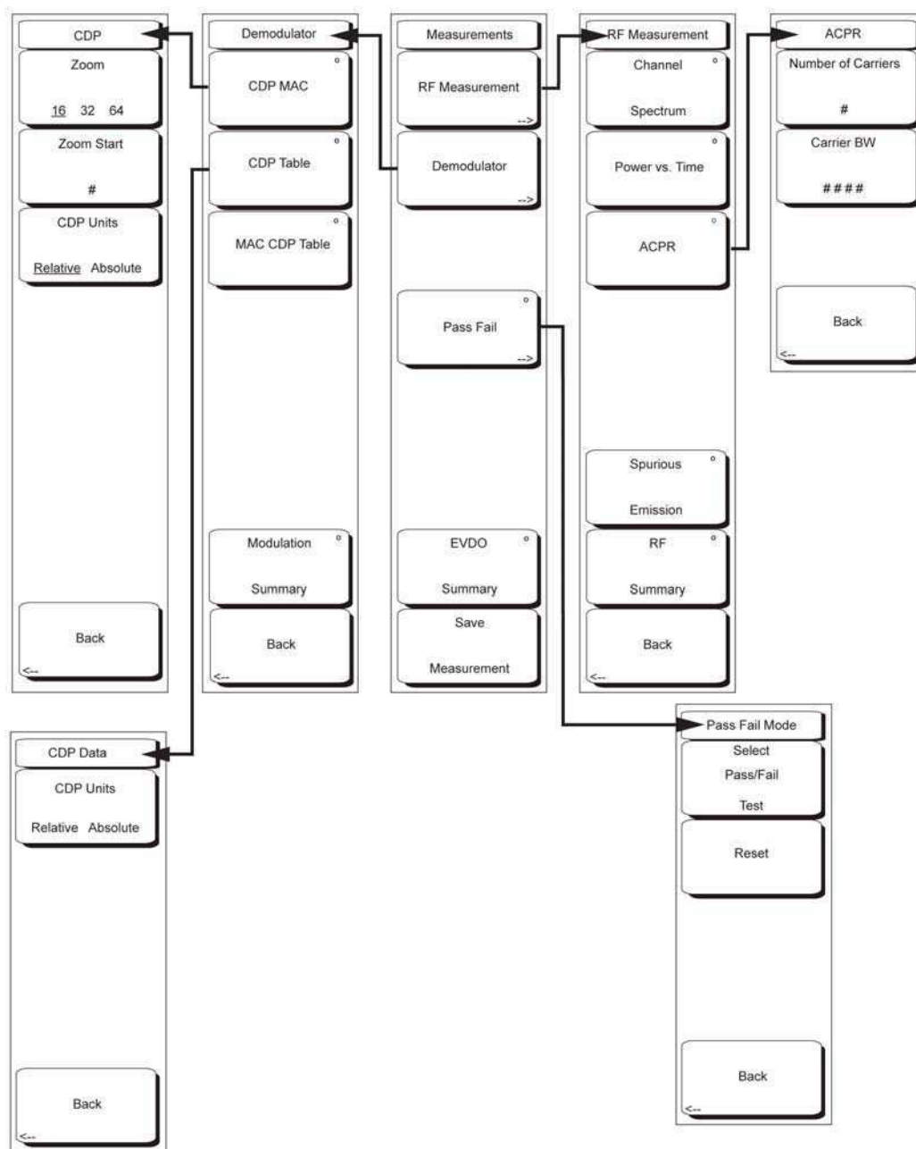
Figure 13-11. EVDO Measurements Menu
