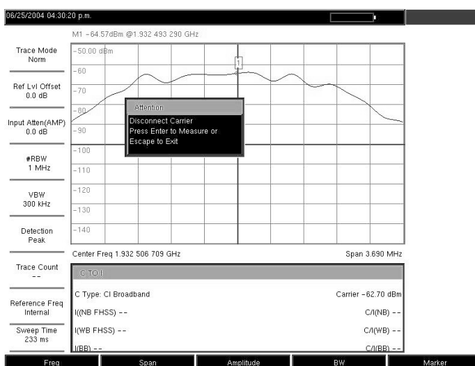
Figure 5-5. C/I Measurement, Carrier Measured
