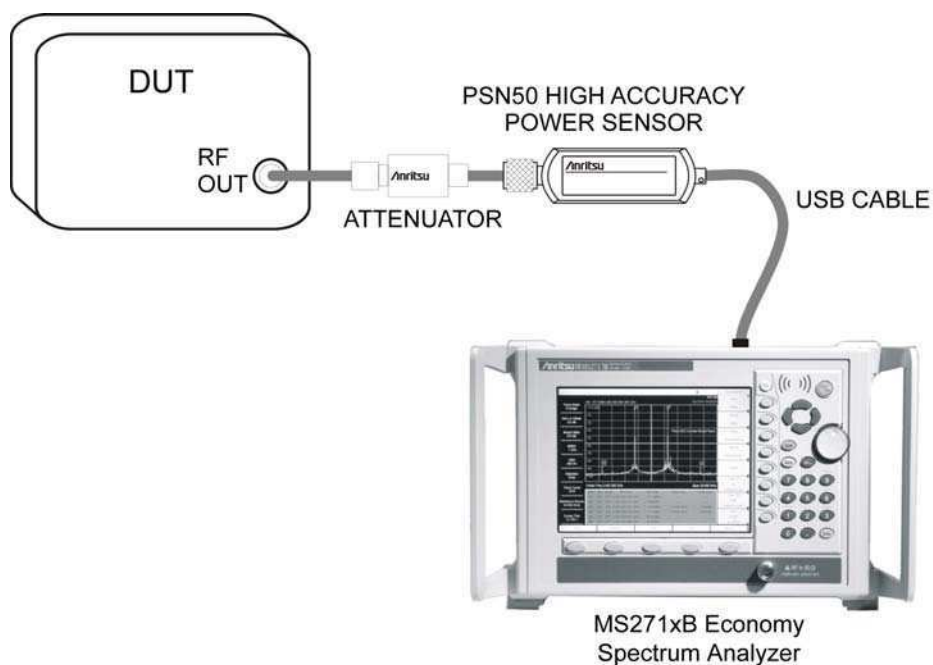
Figure 8-1. High Accuracy Power Meter Setup Example
