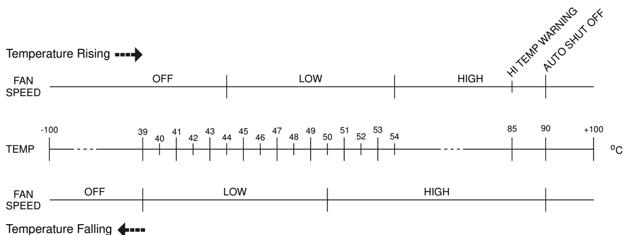
Figure B-1. Fan Speed versus Temperature
