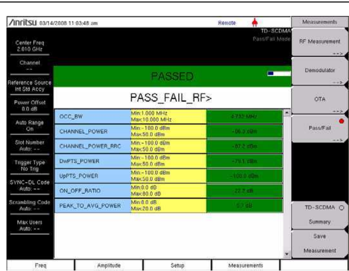
Figure 14-5. Pass/Fail Measurement
