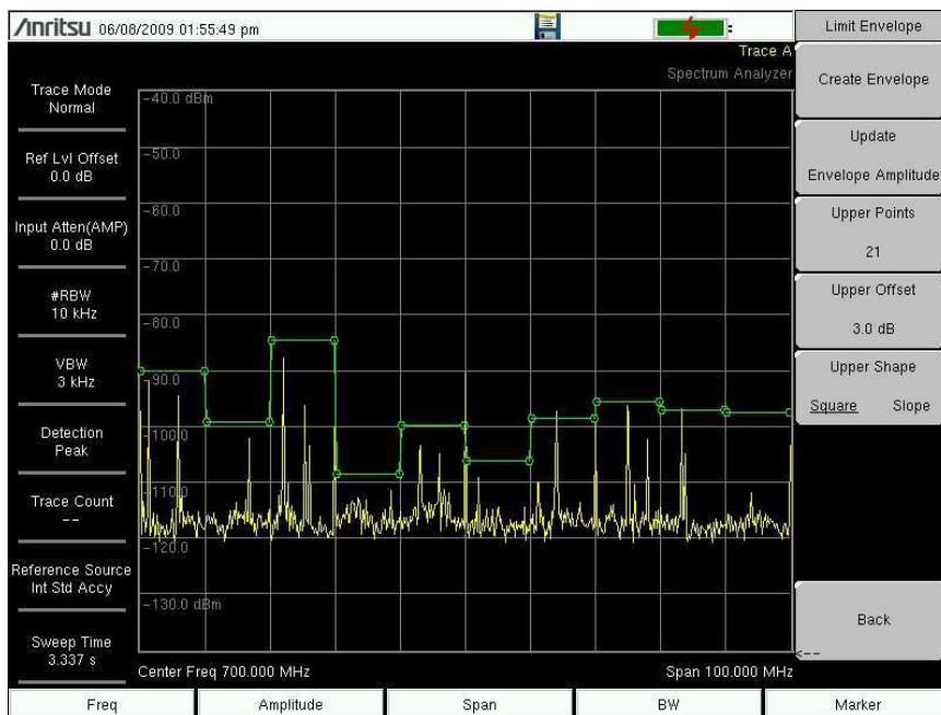
Figure 3-2. Limit Envelope
