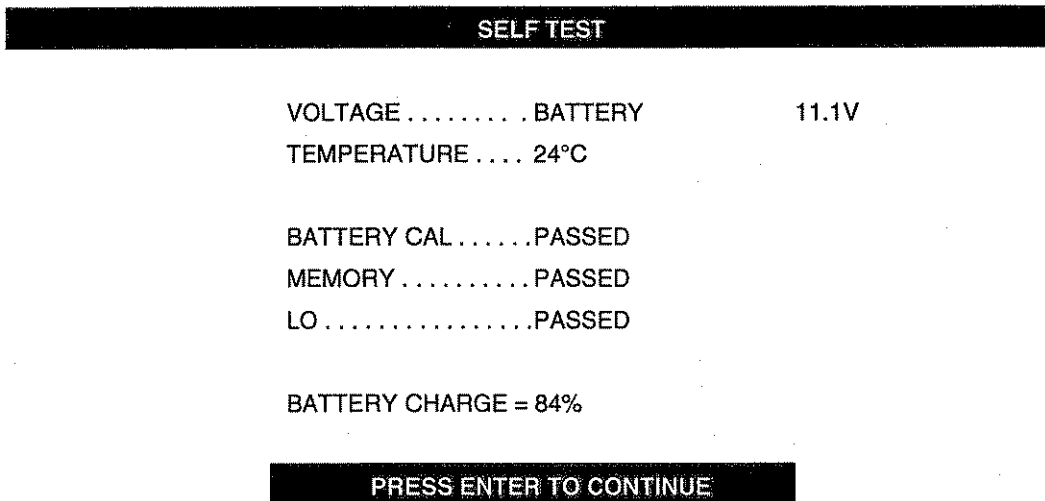
Figure 2-11. Self Test Battery Condition Display
