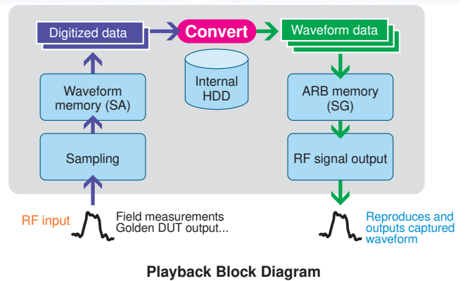
Playback Block Diagram
