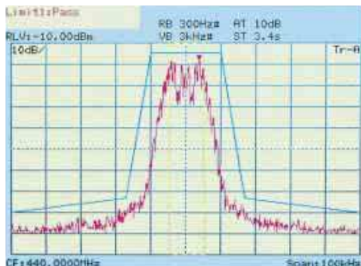
Mask measurement
