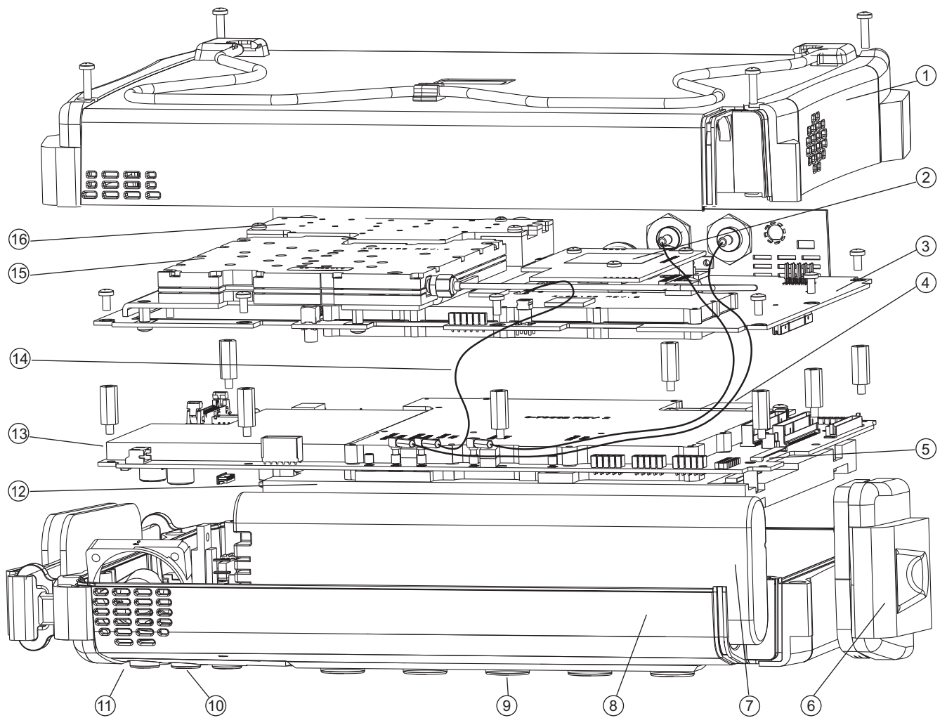
Figure 6-7. VNA Master MS2027C and MS2028C Major Assemblies – Viewed from Bottom
