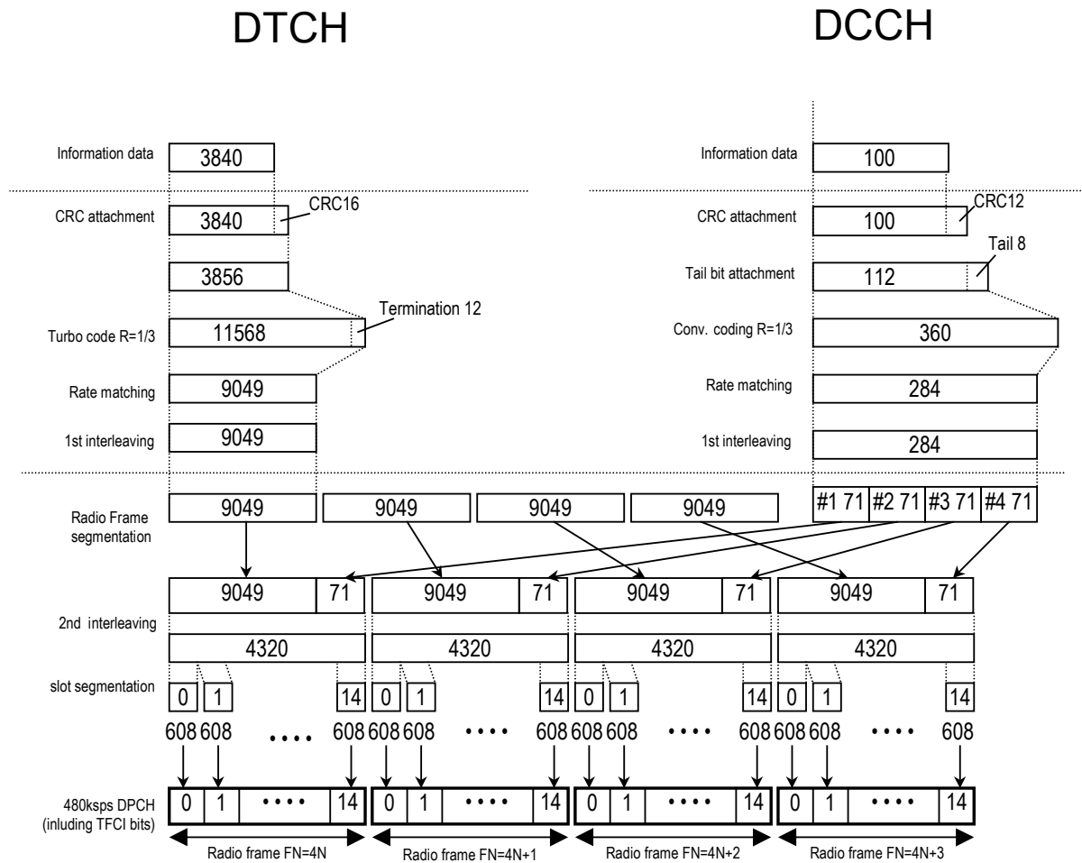
Figure 3.1.4-4 Channel coding for DL reference measurement channel (384 kbps)
