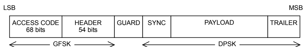
Figure 3.11.2-1 Packet configuration for Enhanced Data Rate waveform
