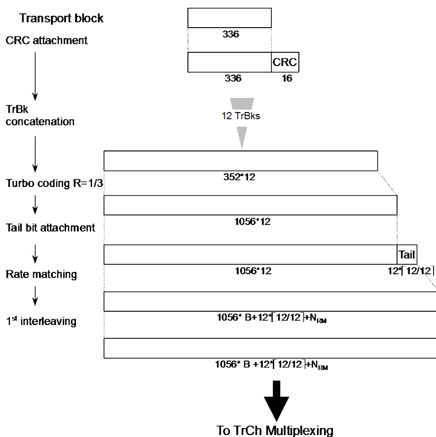
Figure 3.1.5-4 Channel coding for DL 384 kbps packet
