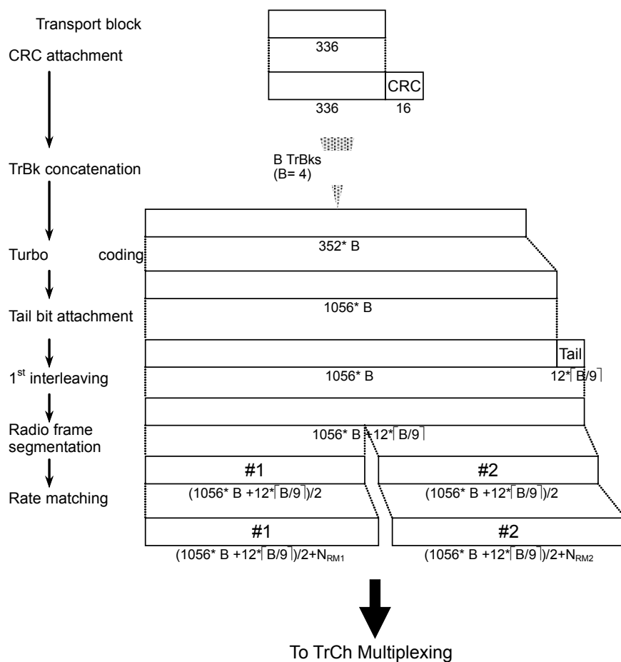
Figure 3.1.2-5 Channel coding for UL 64 kbps packet
