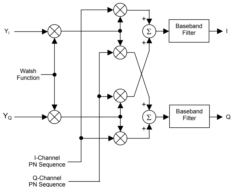
Fig. 3.6.8-2 Signal generation block diagram of waveform pattern FWD_RC3-5 9channel (2/2)
