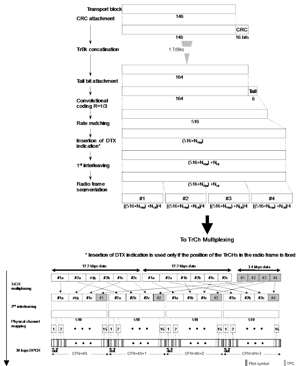
Figure 3.1.5-2 Channel coding and multiplexing for DL AMR TFCSx (2 of 2)
