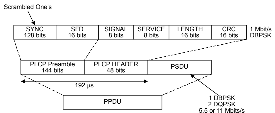
Figure 3.8.2-1 IEEE802.11b Long PLCP PPDU frame format
