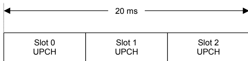
Downlink UPCH 3-slot transmission (DL_Packet_Slot_all)
