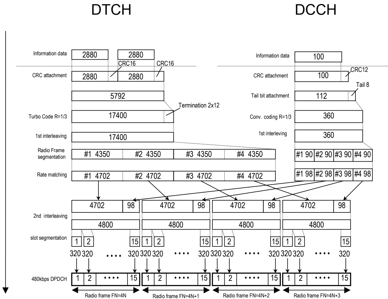
Figure 3.1.1-4 Channel coding for UL reference measurement channel (144 kbps)
