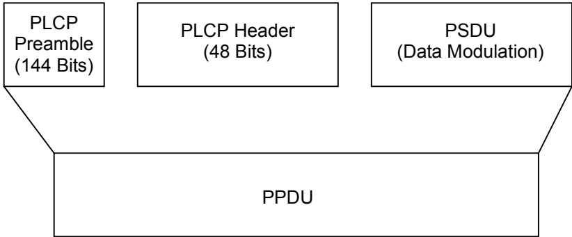
Figure 3.8.3-1 IEEE802.11b Long preamble PPDU frame format
