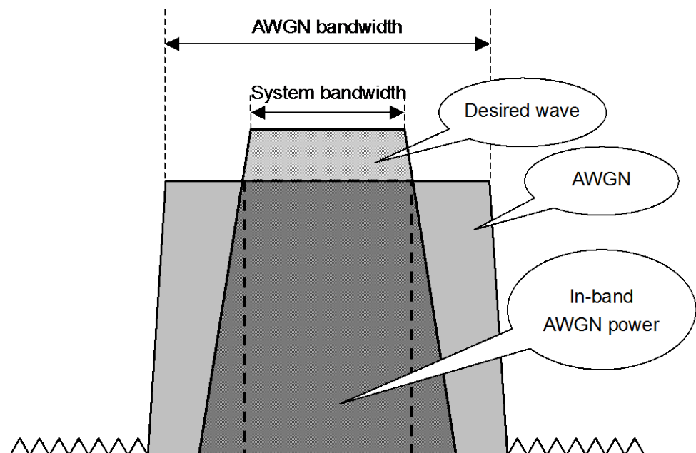
Figure 3.9-1 AWGN bandwidth
