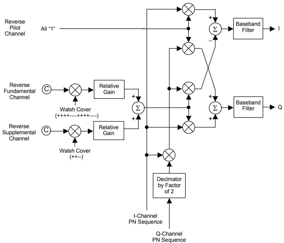
Figure 3.6.4-3 Signal generation block diagram of waveform pattern RVS_RC3_FCH_SCH (2/2)
