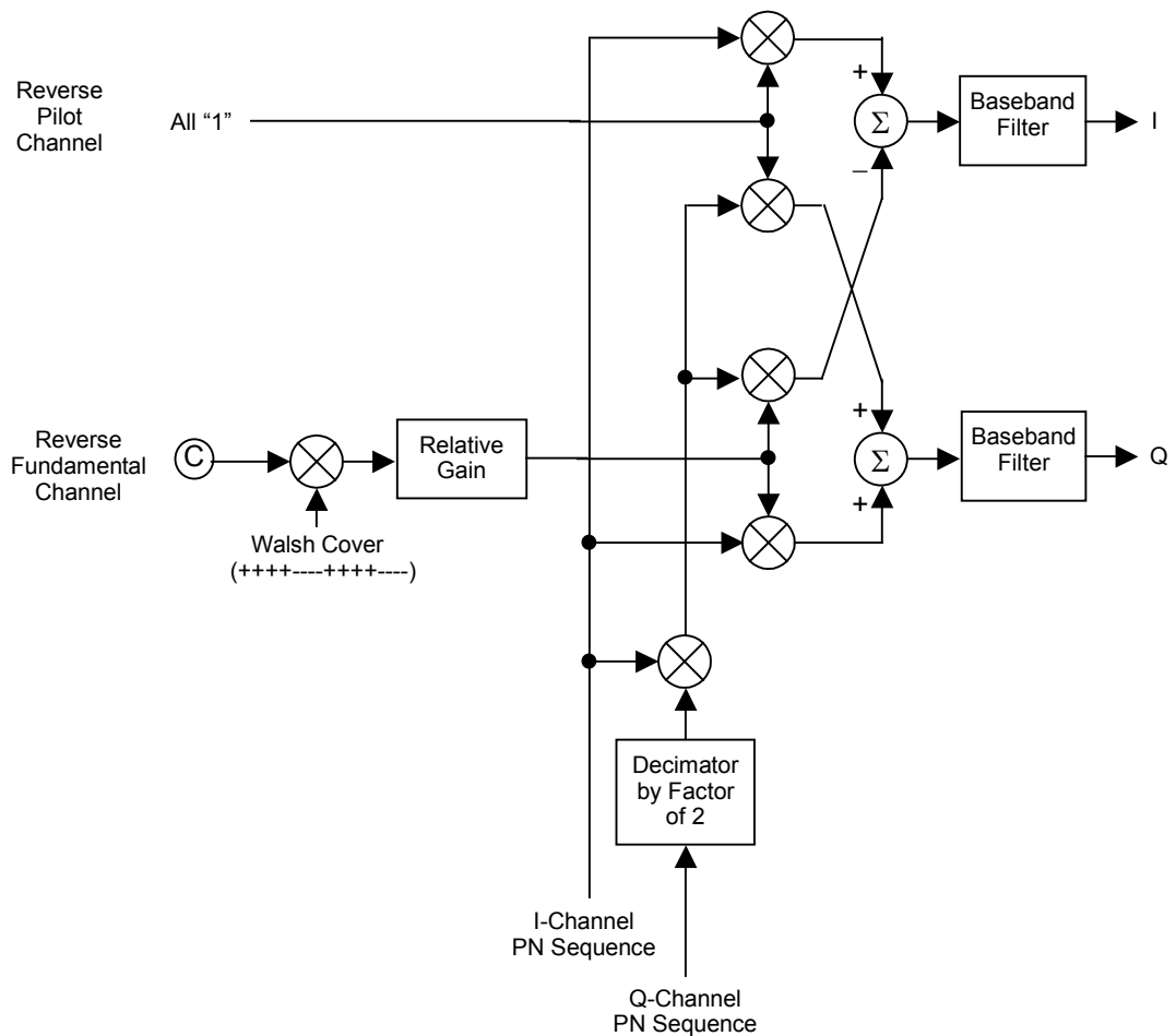
Figure 3.6.6-3 Signal generation block diagram of waveform pattern RVS_RC4_FCH (2/2)
