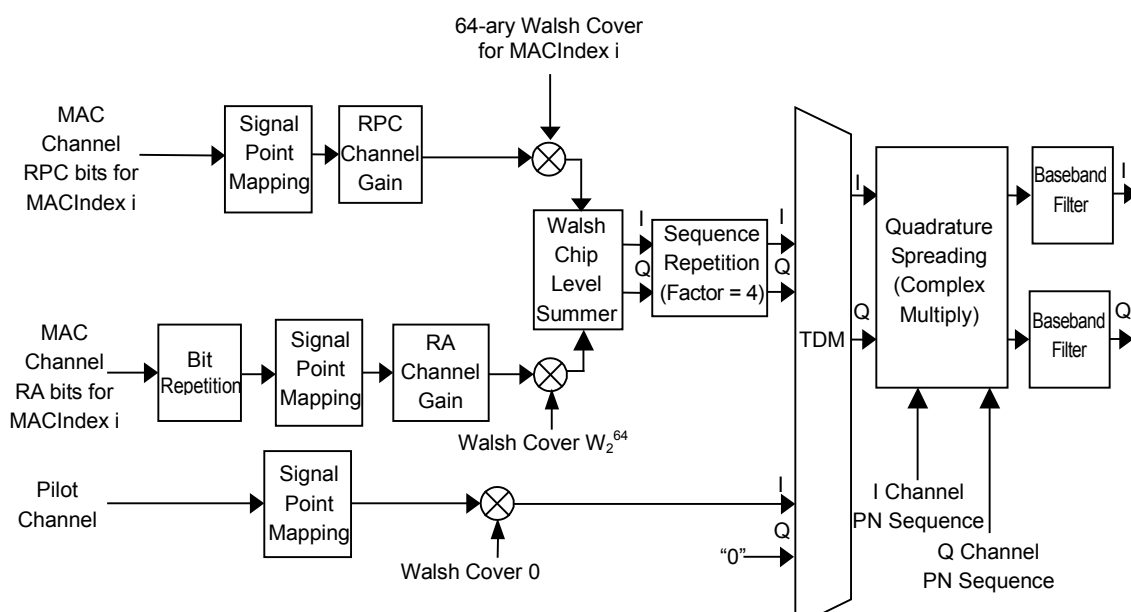
Figure 3.7.3-1 Signal generation block diagram of 1xEV-DO forward idle slot waveform pattern
