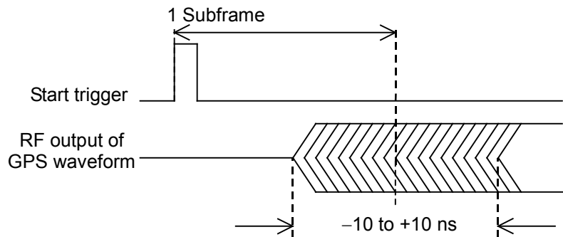
Figure 3.12-1 SYNC_ADJ output timing
