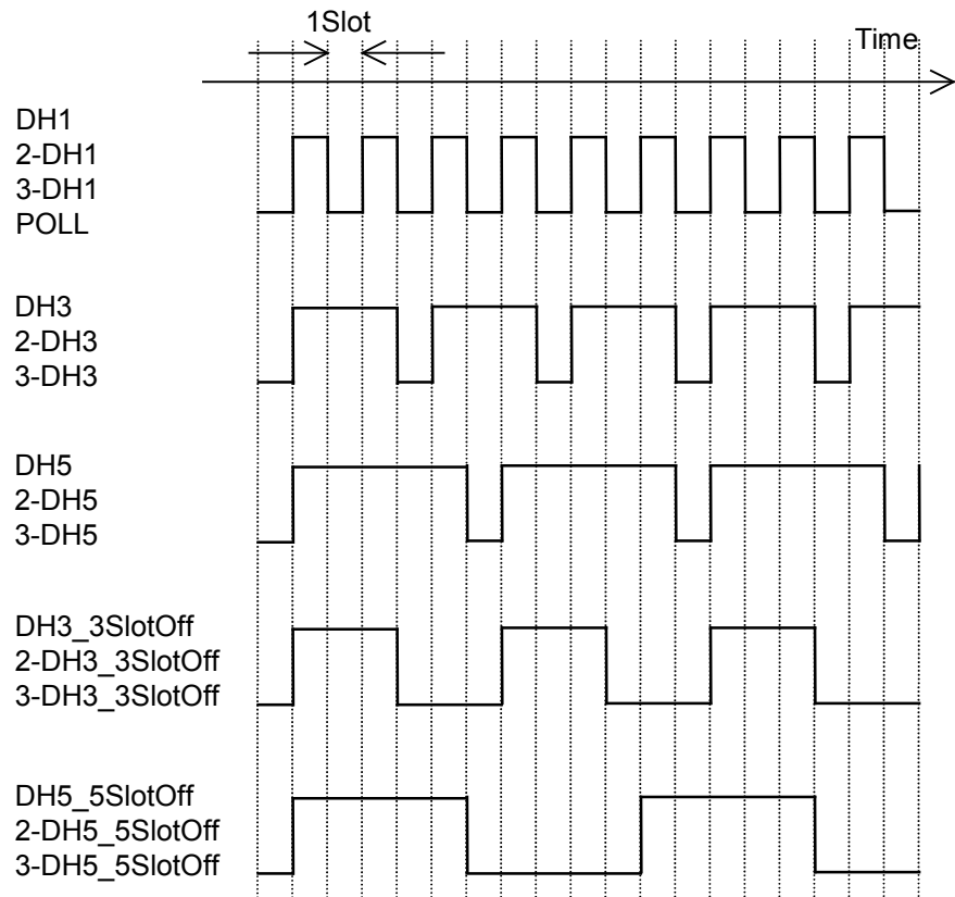
Figure 3.11-1 Timing chart of waveform patterns
