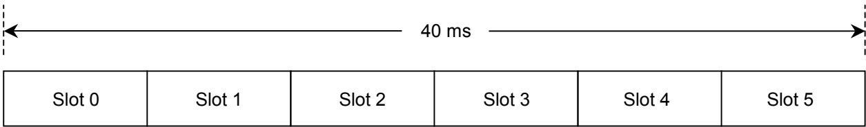
Figure 3.2.1-2 Frame configuration at half rate
