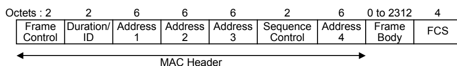
Figure 3.8.1-2 IEEE802.11a MAC frame format
