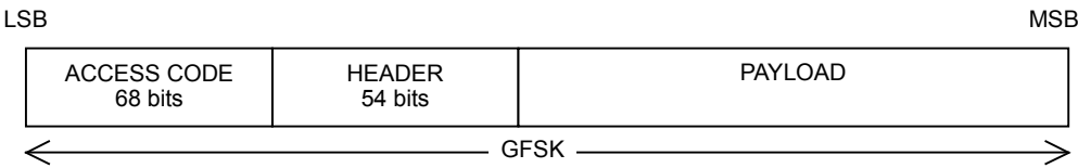
Figure 3.11.1-1 Packet configuration for Basic Rate waveform
