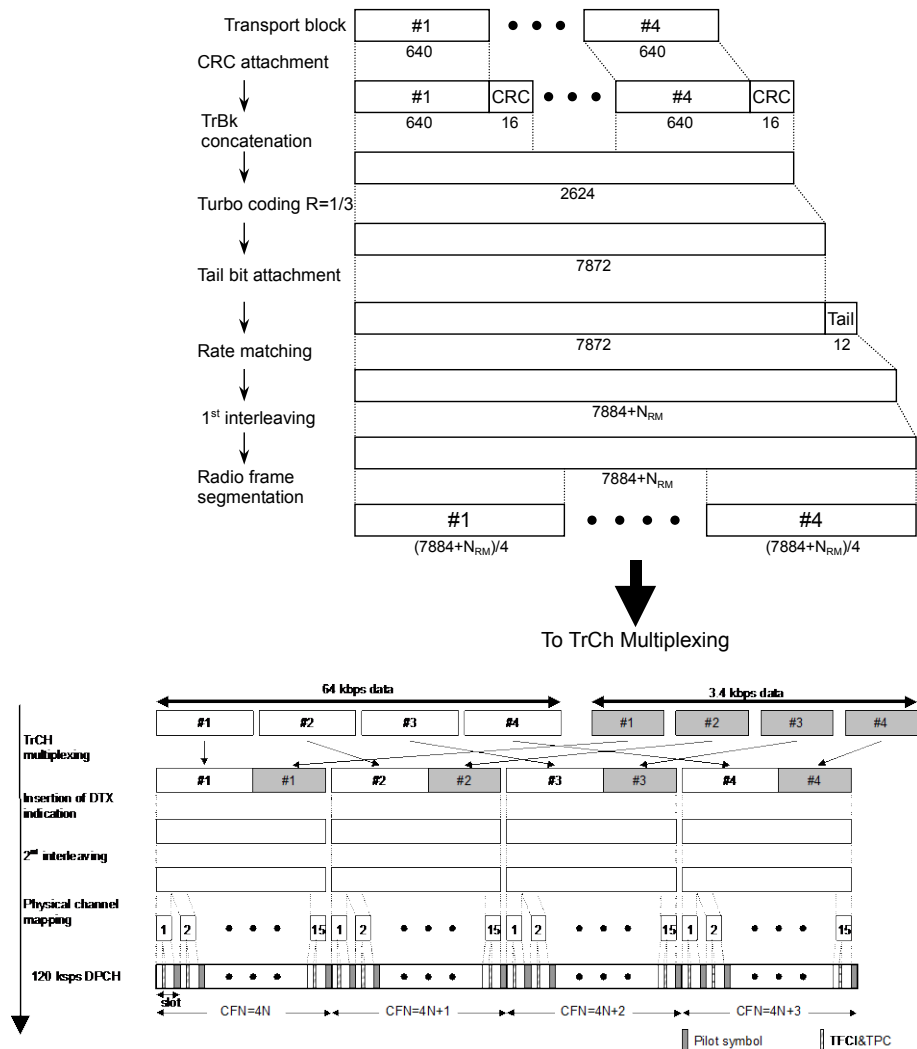
Figure 3.1.5-3 Channel coding and multiplexing for DL ISDN
