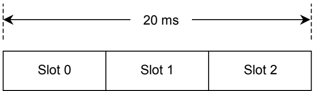
Figure 3.2.1-1 Frame configuration at full rate
