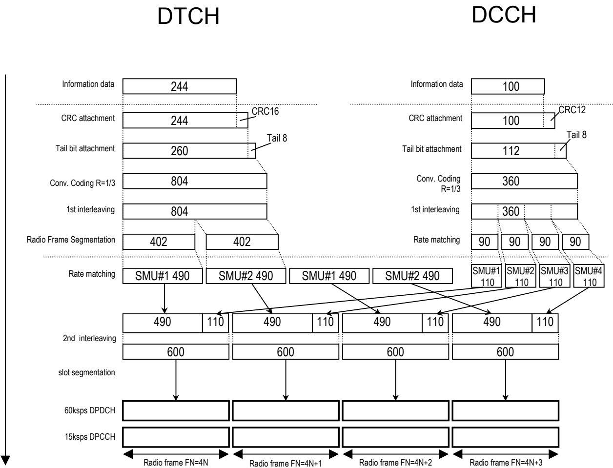
Figure 3.1.1-2 Channel coding for UL reference measurement channel (12.2 kbps)
