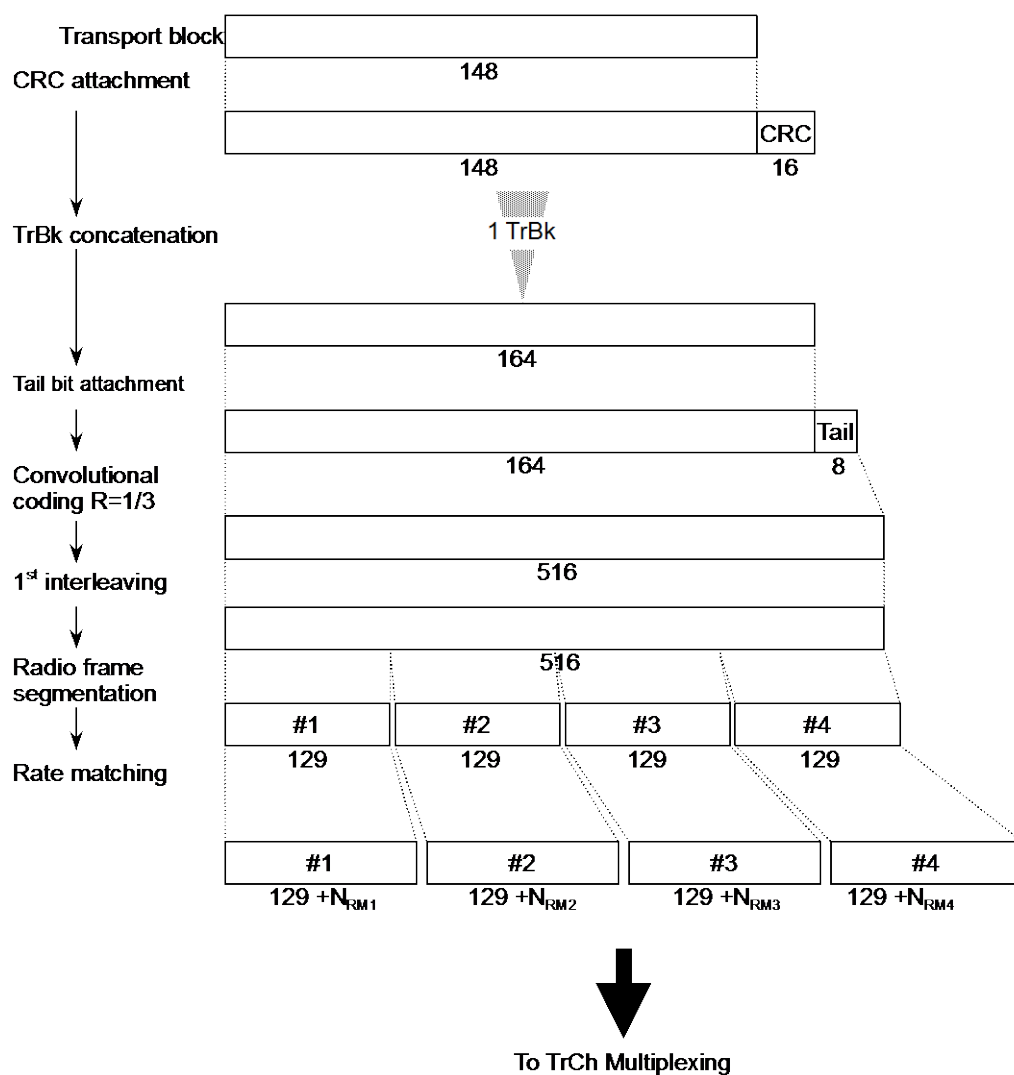
Figure 3.1.2-1 Channel coding and multiplexing for UL AMR TFCSx (1 of 2)
