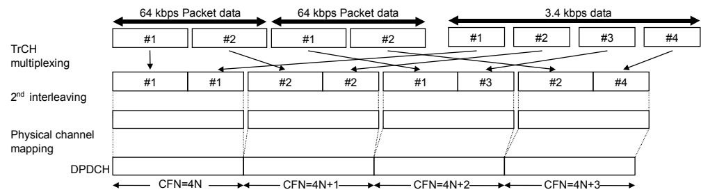
Figure 3.1.2-4 Multiplexing for UL ISDN
