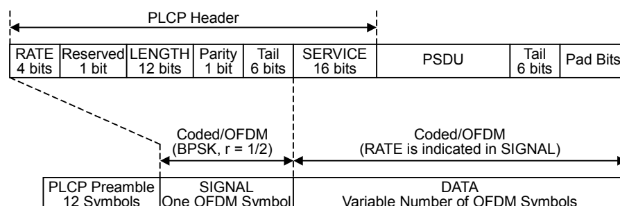
Figure 3.8.1-1 IEEE802.11a PPDU frame format
