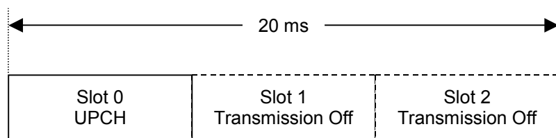
Uplink UPCH 1-slot transmission (UL_Packet_Slot_0)
