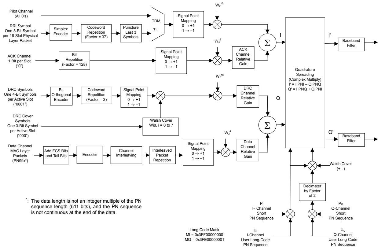
Figure 3.7.2-2 Signal generation block diagram of 1xEV-DO reverse waveform pattern
