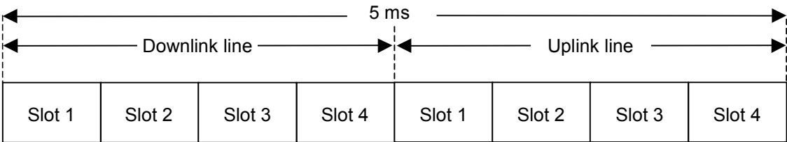
Figure 3.4.1-1 PHS frame configuration
