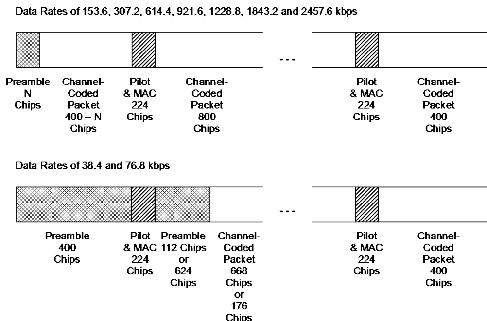
Figure 3.7.1-4 TDM timing diagram
