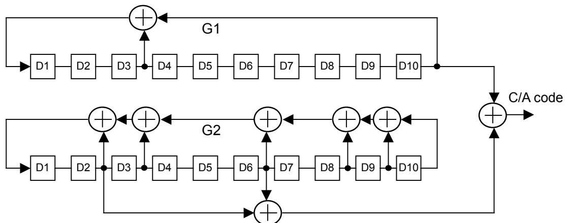
Figure 3.12.1-1 C/A code generation
