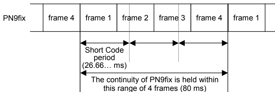
Figure 3.6.1-3 PN9fix data and short code
