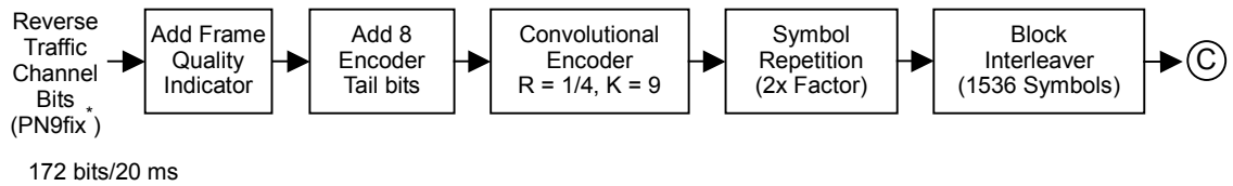
Figure 3.6.3-2 Signal generation block diagram of waveform pattern RVS_RC3_FCH (1/2)
