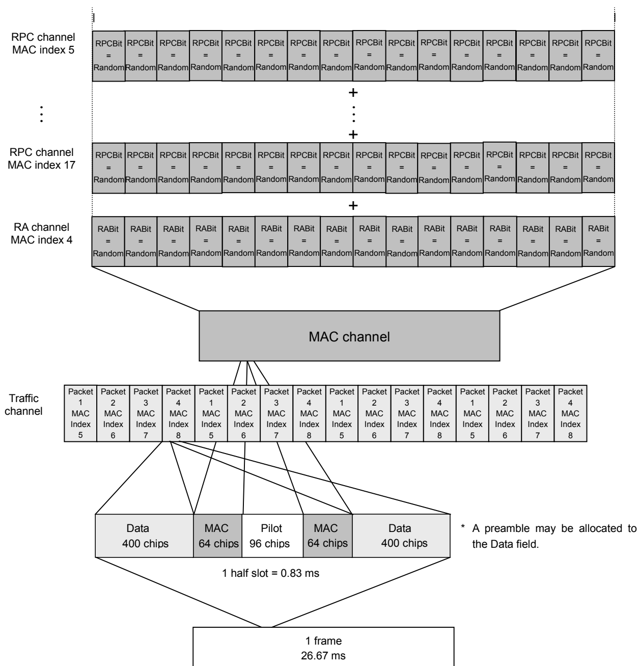
Figure 3.7.1-5 Multiplexing channels
