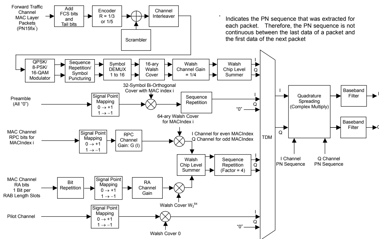
Figure 3.7.1-2 Signal generation block diagram of 1xEV-DO forward waveform pattern
