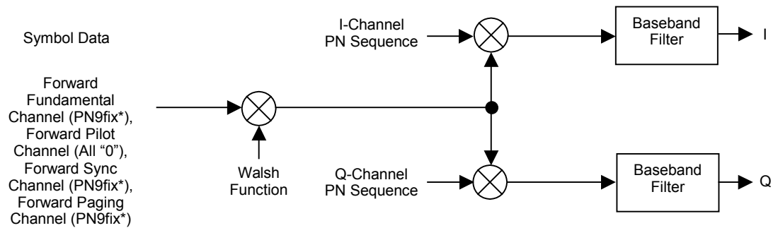
Figure 3.6.7-1 Signal generation block diagram of waveform pattern FWD_RC1-2 9channel
