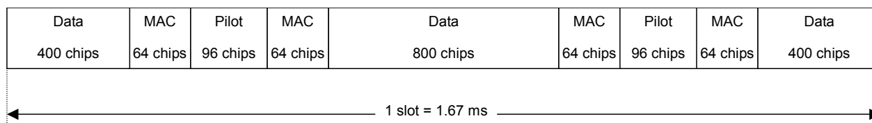
Figure 3.7.1-3 Slot format of 1xEV-DO forward waveform pattern (excluding idle slot)
