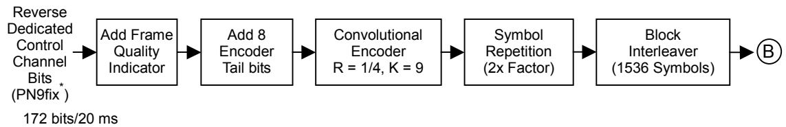
Figure 3.6.5-2 Signal generation block diagram of waveform pattern RVS_RC3_DCCH (1/2)
