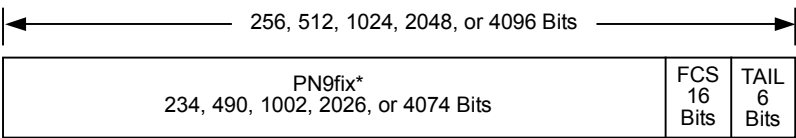
Figure 3.7.2-1 Format of 1xEV-DO reverse packet
