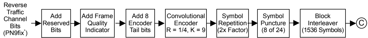
Figure 3.6.6-2 Signal generation block diagram of waveform pattern RVS_RC4_FCH (1/2)
