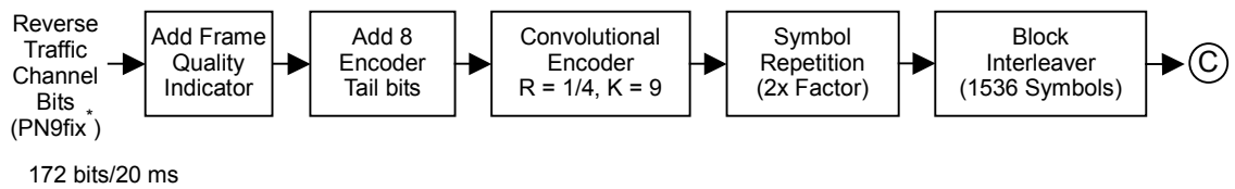
Figure 3.6.4-2 Signal generation block diagram of waveform pattern RVS_RC3_FCH_SCH (1/2)
