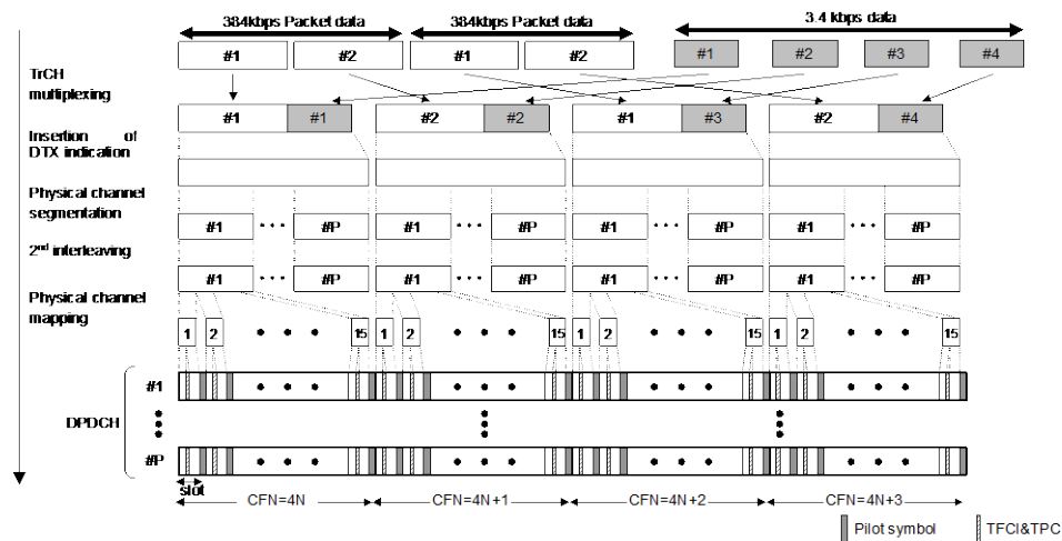
Figure 3.1.5-5 Multiplexing for DL 384 kbps
