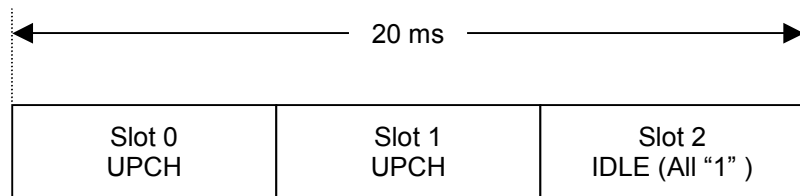
Downlink UPCH 2-slot transmission (DL_Packet_Slot_01)
