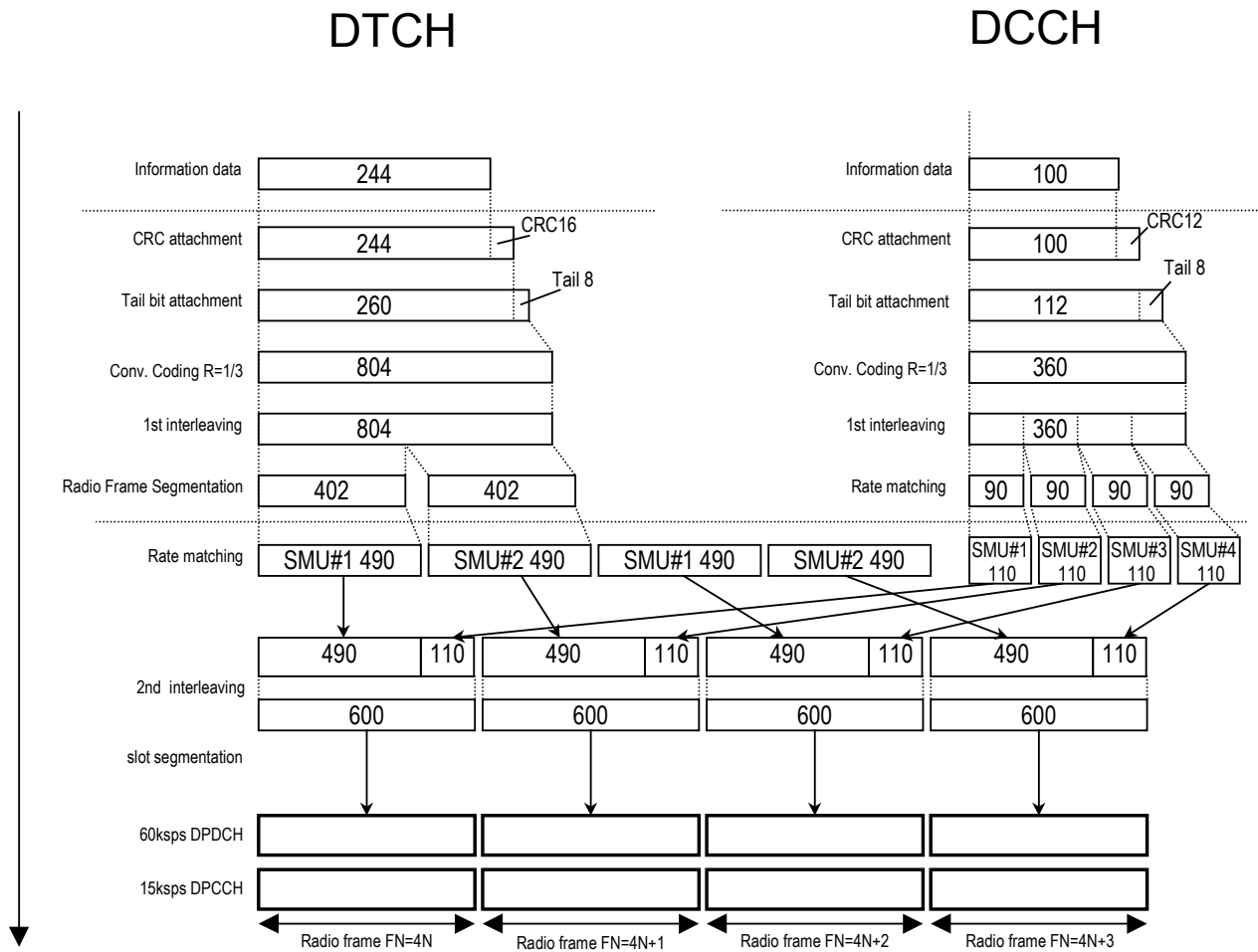
Figure 3.1.1-1 Channel coding for UL reference measurement channel (12.2 kbps)
