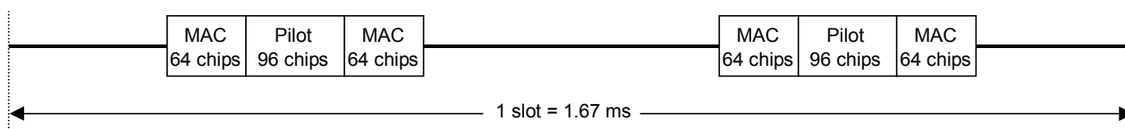
Figure 3.7.3-2 Format of 1xEV-DO forward idle slot waveform pattern
