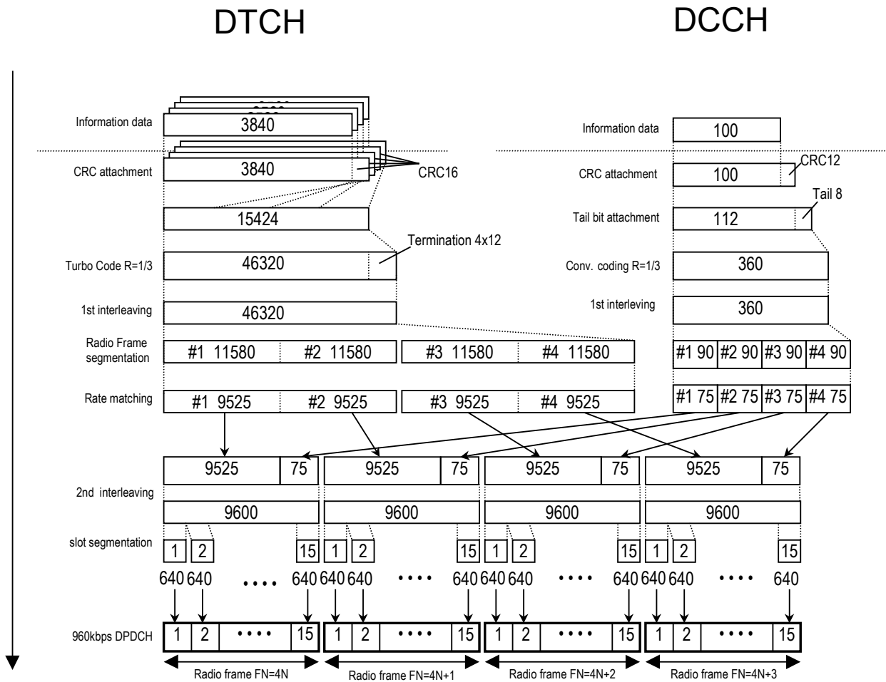
Figure 3.1.1-5 Channel coding for UL reference measurement channel (384 kbps)
