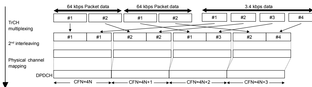
Figure 3.1.2-6 Multiplexing for UL 64 kbps packet
