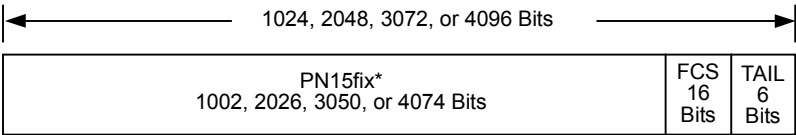
Figure 3.7.1-1 Format of 1xEV-DO forward packet
