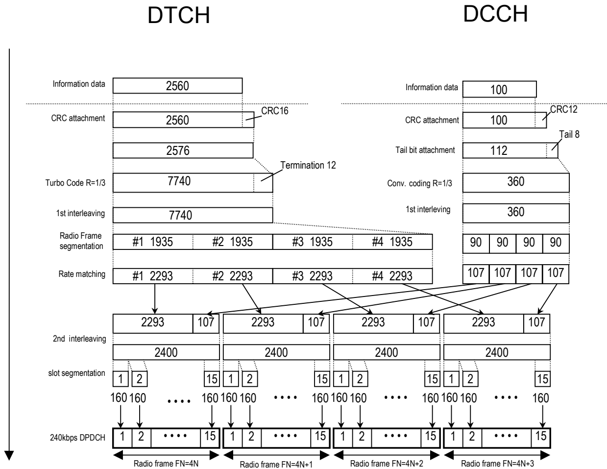
Figure 3.1.1-3 Channel coding for UL reference measurement channel (64 kbps)
