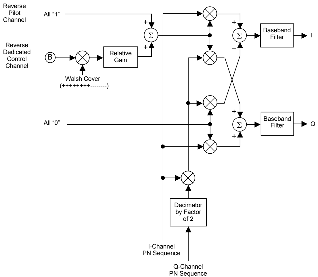
Figure 3.6.5-3 Signal generation block diagram of waveform pattern RVS_RC3_DCCH (2/2)
