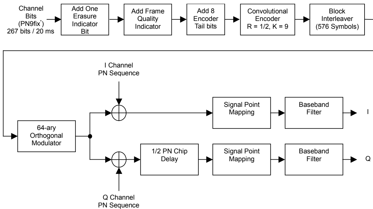
Figure 3.6.2-2 Signal generation block diagram of waveform pattern RVS_RC2_FCH
