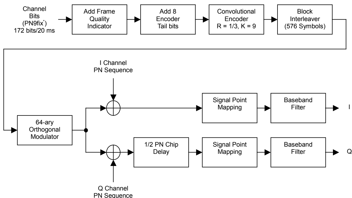
Figure 3.6.1-2 Signal generation block diagram of waveform pattern RVS_RC1_FCH
