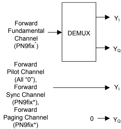
Figure 3.6.8-1 Signal generation block diagram of waveform pattern FWD_RC3-5 9channel (1/2)
