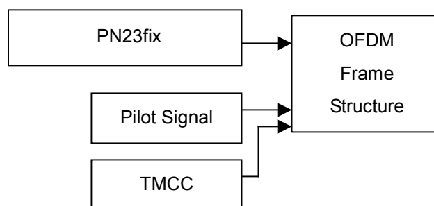
Figure 3.10.1-2 Generation of the waveform patterns for ISDB-T
