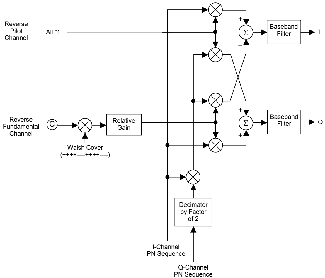
Figure 3.6.3-3 Signal generation block diagram of waveform pattern RVS_RC3_FCH (2/2)
