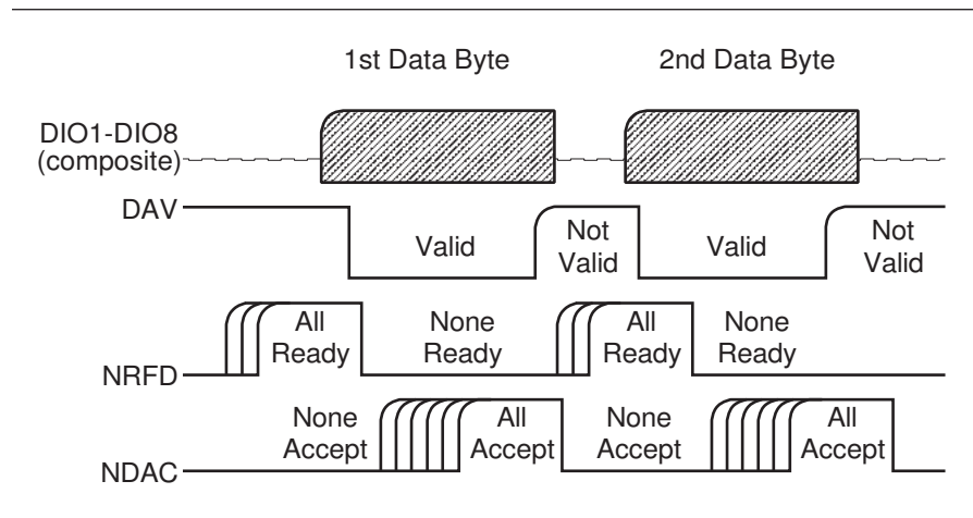
Figure 1-2. Typical GPIB Handshake Operation
