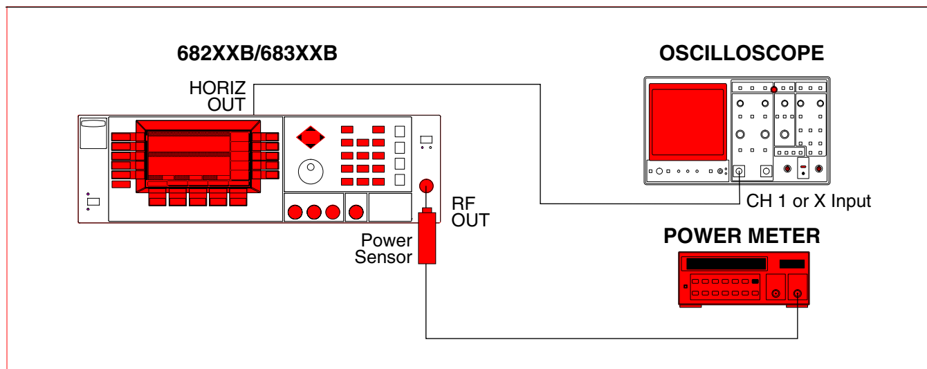
Figure 5-2. Equipment Setup for Power Level Accuracy and Flatness Tests
