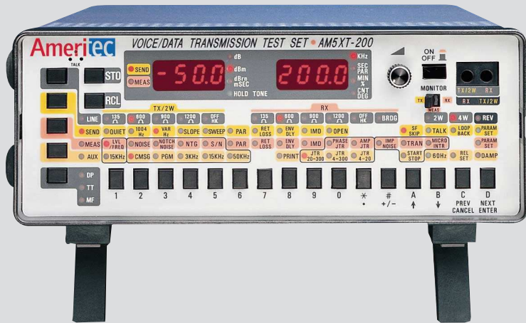
Model AM5XT-200 / IEEE 743-1984 Standard / 200kHz Bandwidth
