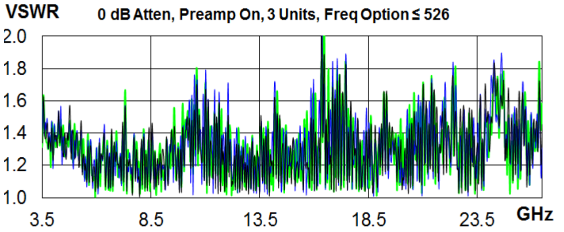
Nominal VSWR – Preamp On Band [Plot]
