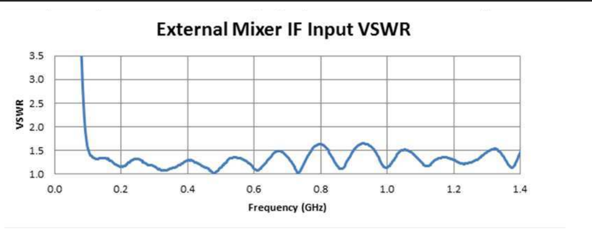
External Mixer IF Input VSWR [Plot]
