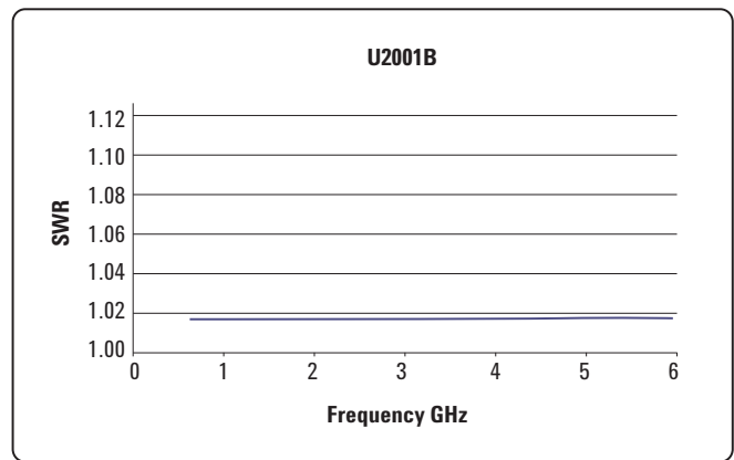
Typical SWR for U2001B sensor (25 °C ± 10 °C)
