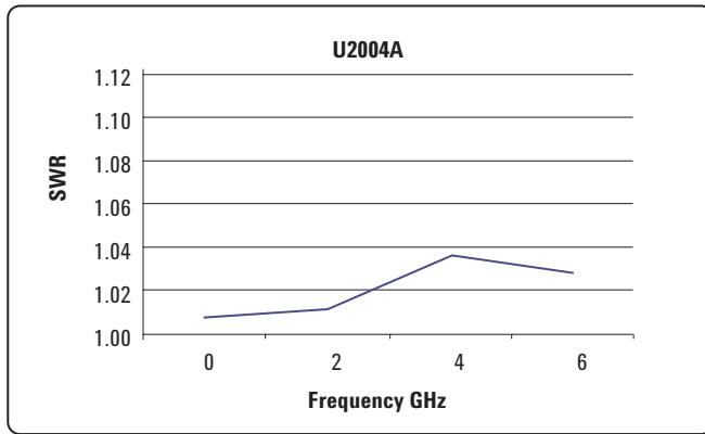
Typical SWR for U2004A sensor (25 °C ± 10 °C)
