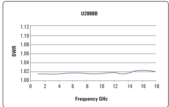
Typical SWR for U2000B sensor (25 °C ± 10 °C)
