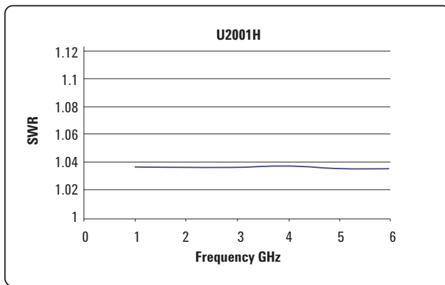
Typical SWR for U2001H sensor (25 °C ± 10 °C)
