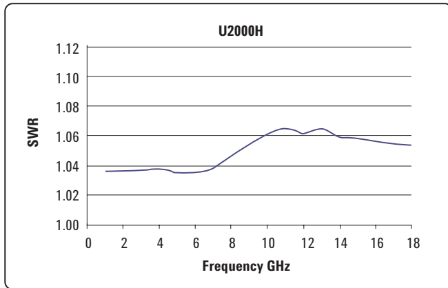
Typical SWR for U2000H sensor (25 °C ± 10 °C)
