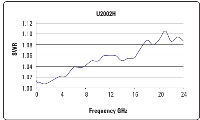
Typical SWR for U2002H sensor (25 °C ± 10 °C)
