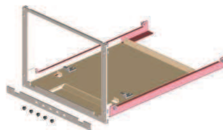
Mount your 9000 Series scope in an 8U high, 19" (487mm) wide rack with option 1CM.
