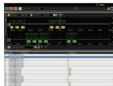
Trigger on and decode RS-232/UART transmission.
