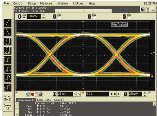
8 Gb/s real-time eye diagram with DS081204A
