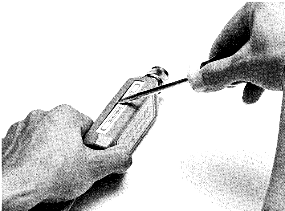
Figure 4-1. Cover Removal
