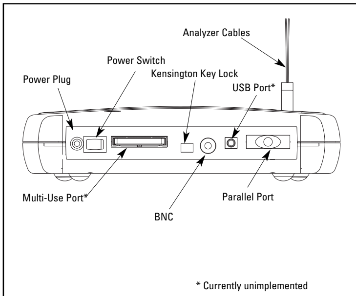
Figure 5. Diagram of LogicWave rear panel
