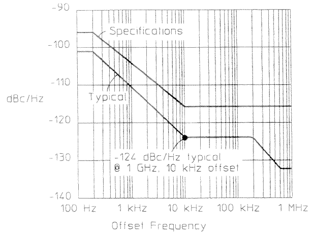
Spectral purity at 1 GHz
