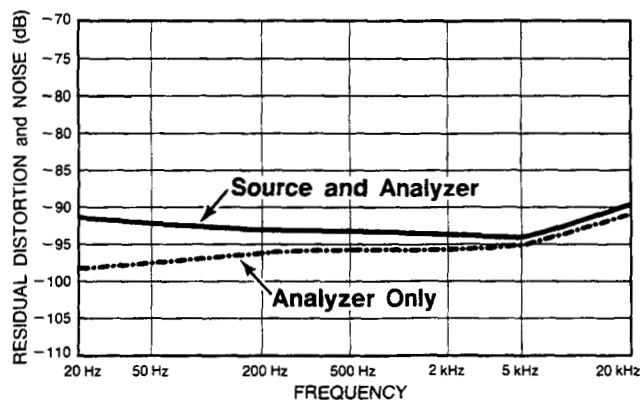
Figure 1-2. Typical Combined Source and Analyzer Residual Distortion With V_{source} Set to 1.5V (80 kHz BW)
