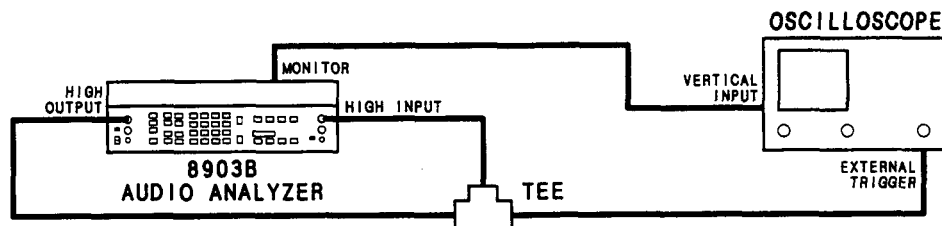
Figure 5-3. Notch Filter Tune and Balance Adjustment Test Setup
