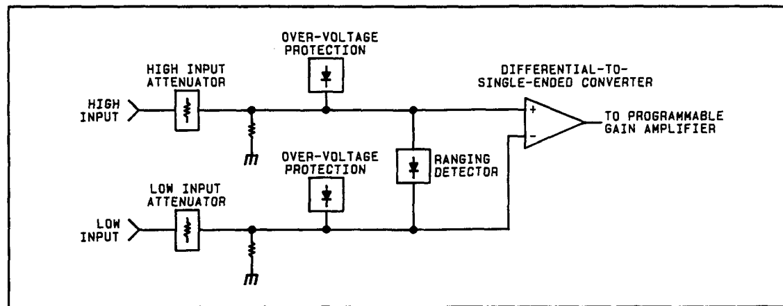
Analyzer Input Block Diagram
