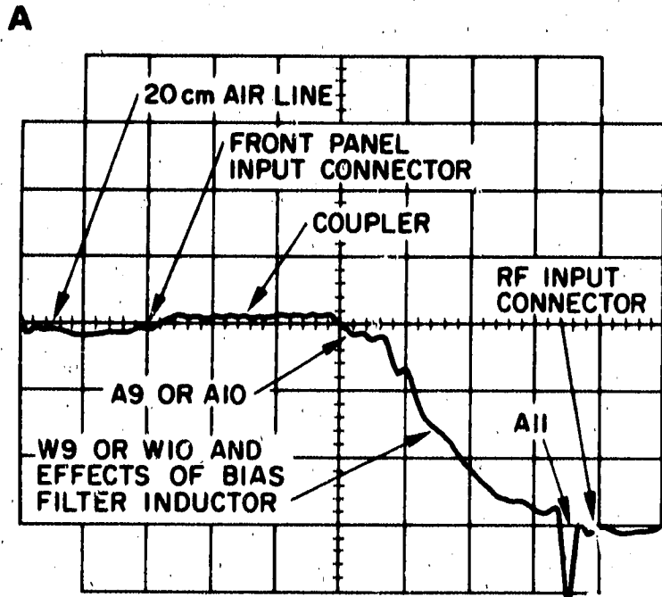
Normal Display looking into INPUT PORT A or INPUT PORT B with RF INPUT terminated in 50 Ω and Bias Input shorted to chassis.
