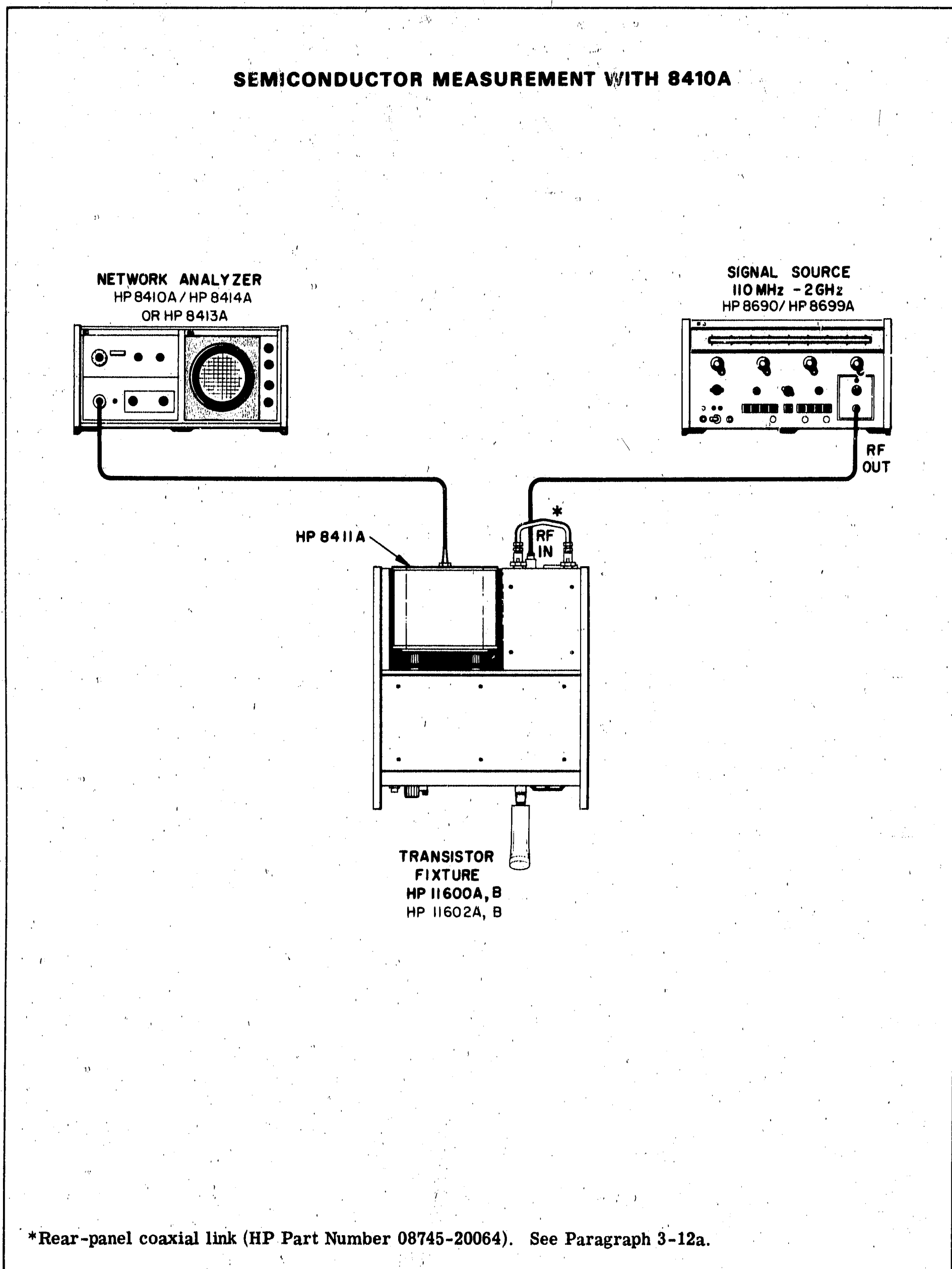
Figure 3-11. Semiconductor Measurement with 8410A Network Analyzer Readout (Sheet 1 of 2)
