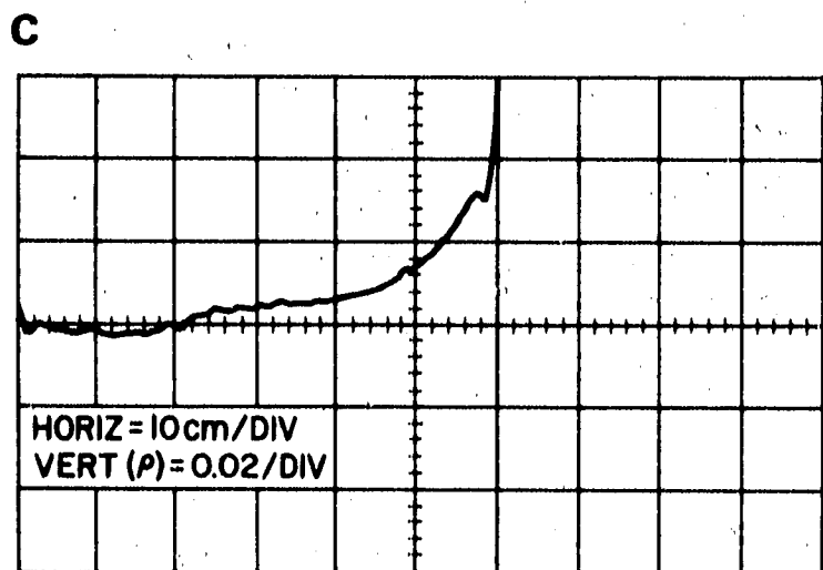
Normal Display looking into INPUT PORT A or INPUT PORT B with RF INPUT terminated in 50 Ω and Bias Input shorted to chassis.
