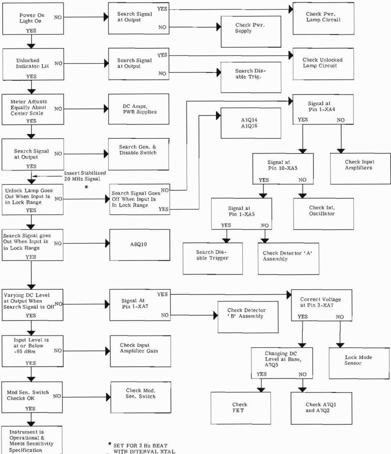
Figure 5-5. Functional Troubleshooting Flow Chart
