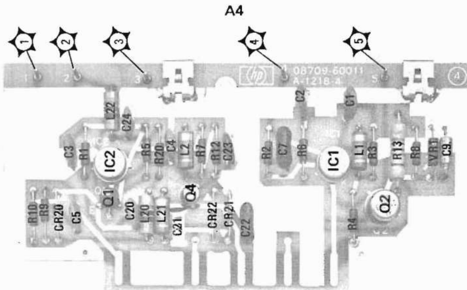
Figure 7-8a. A4 Amplifier Board Assembly Component Identification and Location (CHANGE 5)
