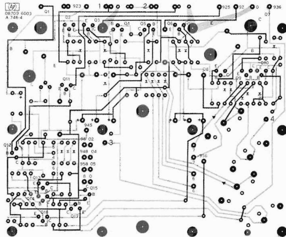
Figure 7-6b. A1 Power Supply/Amplifier Board Assembly Output Amplifier and Light Amplifier Circuit Paths and Solder Pads
