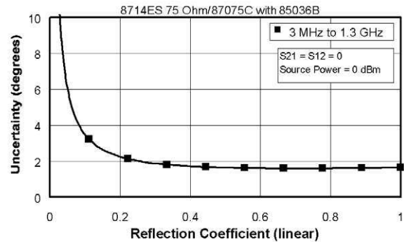
Phase, ET models with attenuator
