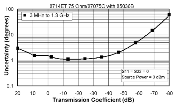
Phase, ET models without attenuator
