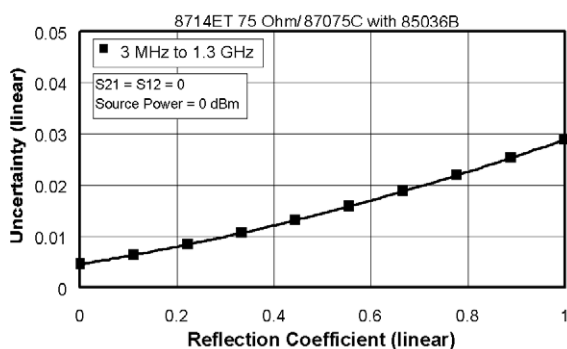
Magnitude, ET models without attenuator
