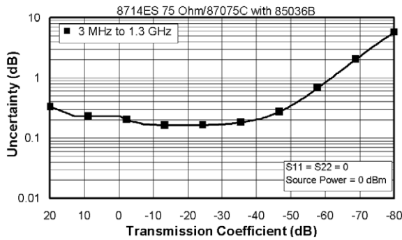
Magnitude, ET models with attenuator
