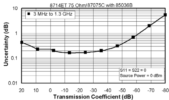
Magnitude, ET models without attenuator
