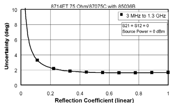
Phase, ET models without attenuator
