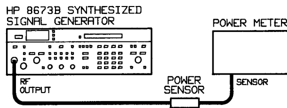
Figure 4-2. Output Level and Flatness Test Setup
