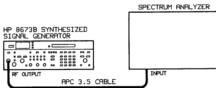
Figure 4-18. Harmonics, Subharmonics, and Multiples Test Setup
