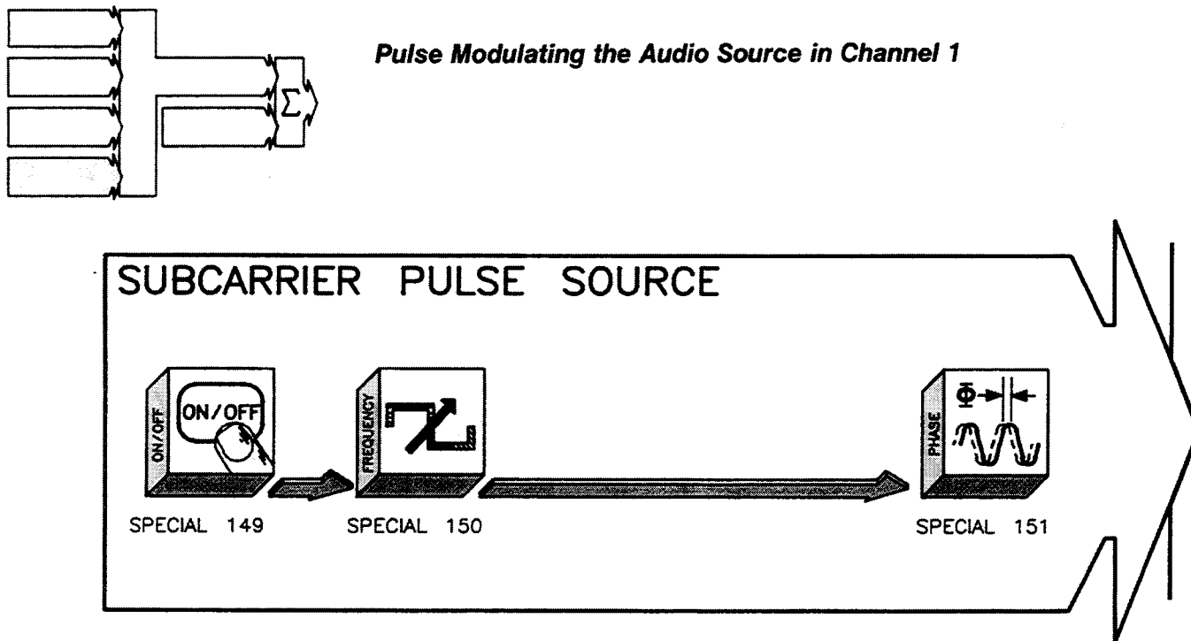
Figure H-9. Block Diagram of the Subcarrier Pulse Source.
