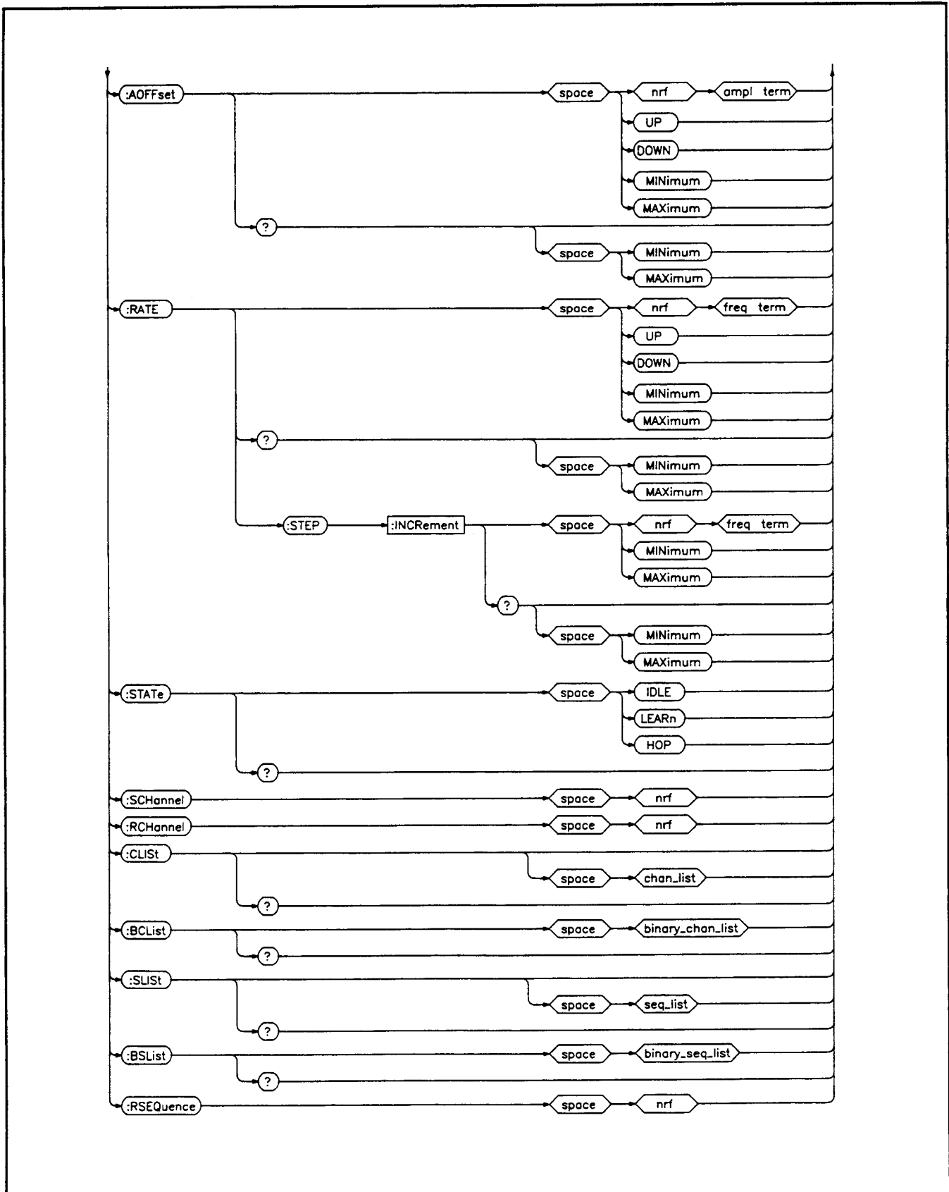
Figure F-9. Frequency Hop Subsystem. (2 of 2)
