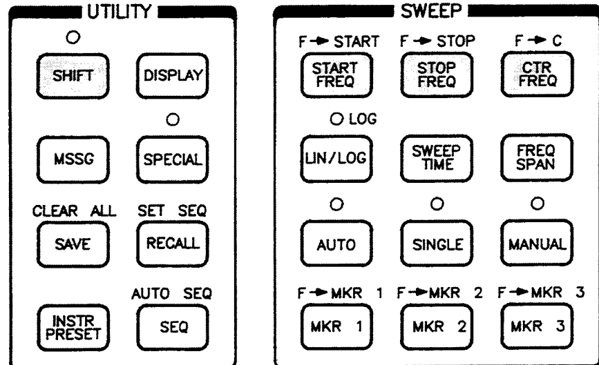
Figure 4-6. Shift Key for Start, Stop, Center, and Span.
