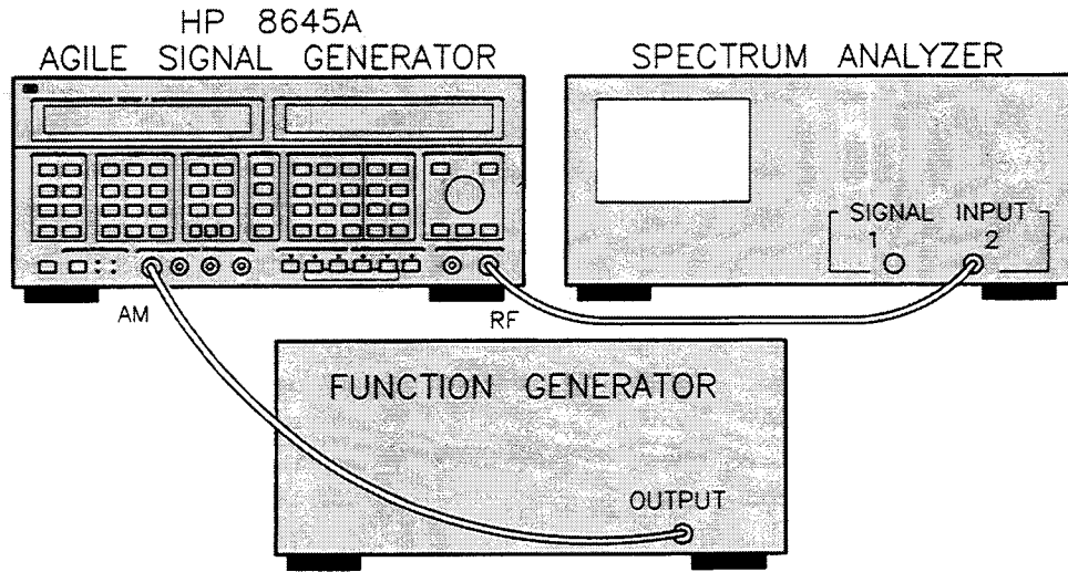
Figure 2-8. Equipment Setup for Simultaneous FM and AM Procedure.
