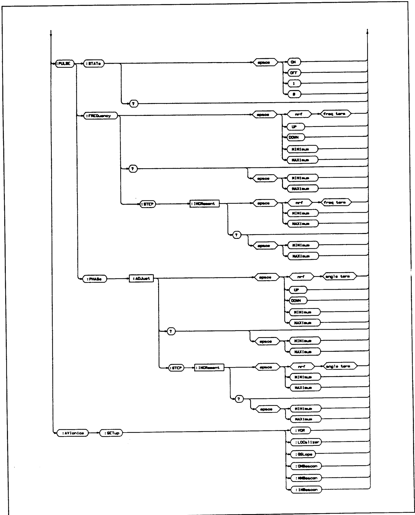
Figure F-13. LF Source Subsystem. (6 of 6)
