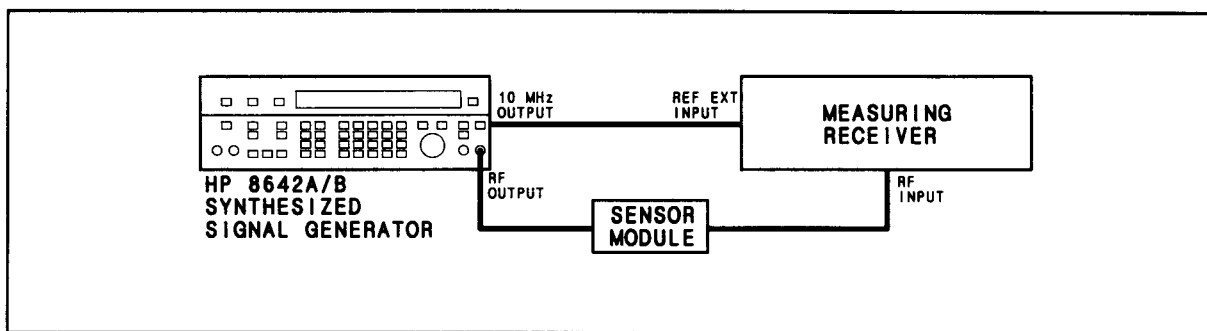
Figure 4-2. Harmonics Test Setup
