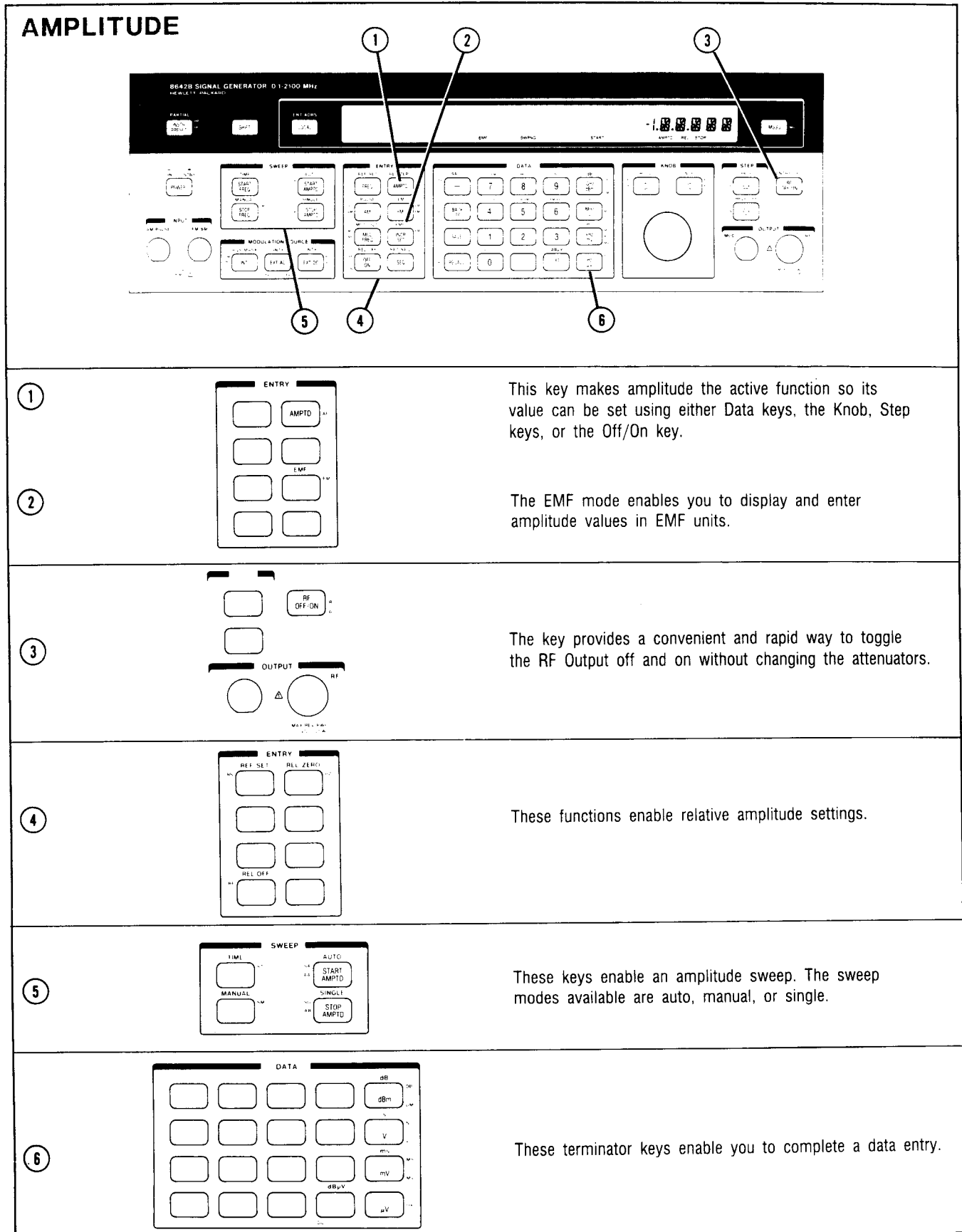
Figure 3-8. Amplitude-Related Functions
