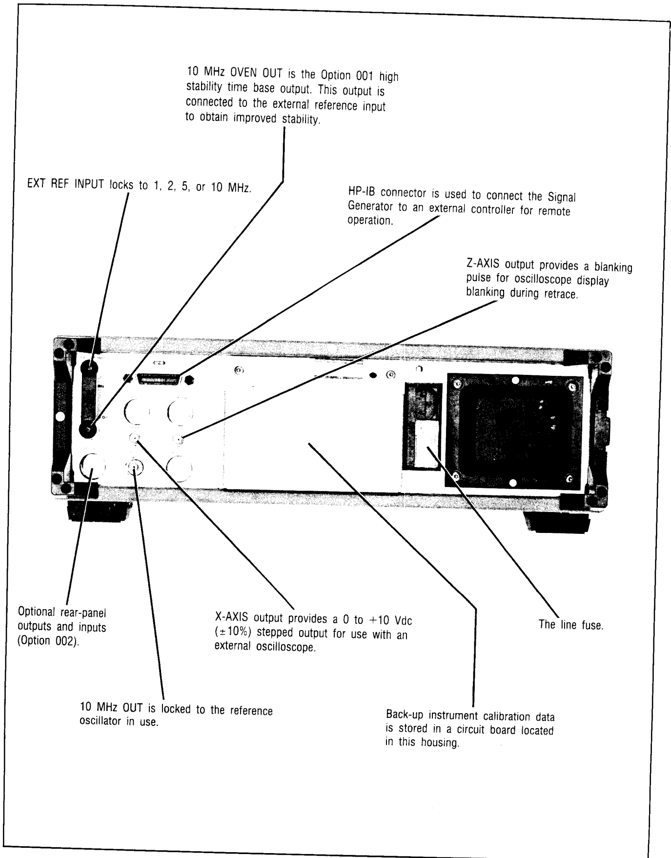
Figure 3-2. Rear-Panel Features
