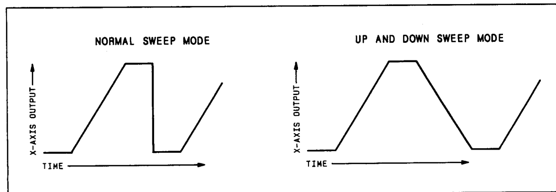
Figure 3-10. Sweep Waveforms
