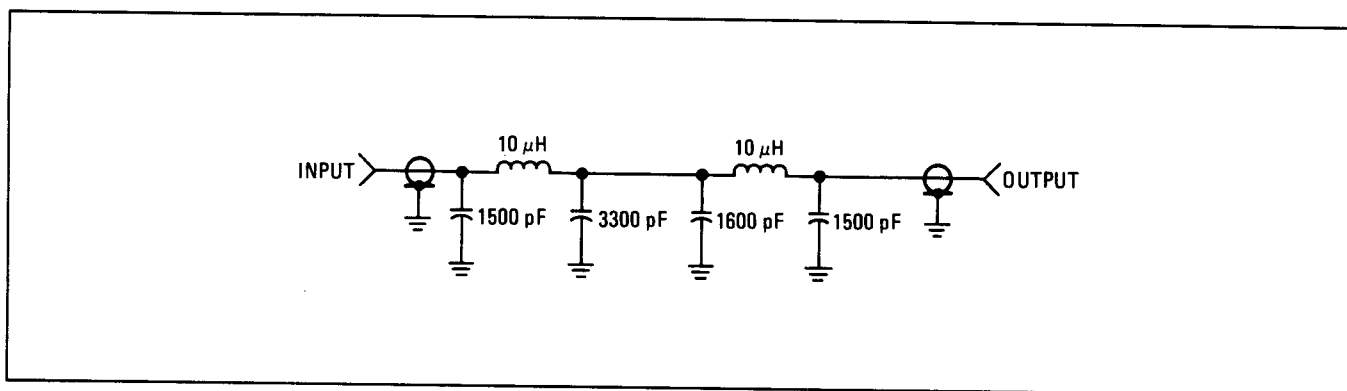
Figure 1-1. 1 MHz Low-Pass Filter
