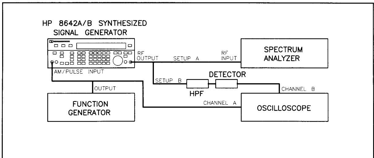
Figure 4-13. Pulse Test Setup
