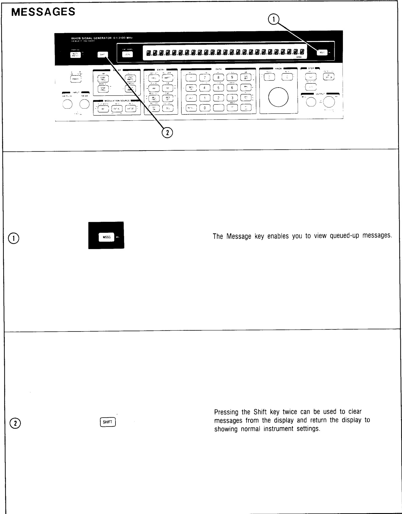
Figure 3-19. Message-Related Keys
