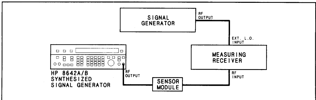
Figure 4-14. Residual Test Setup
