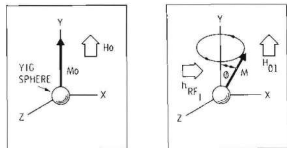
Figure 8-3. Net Magnetization Vector
