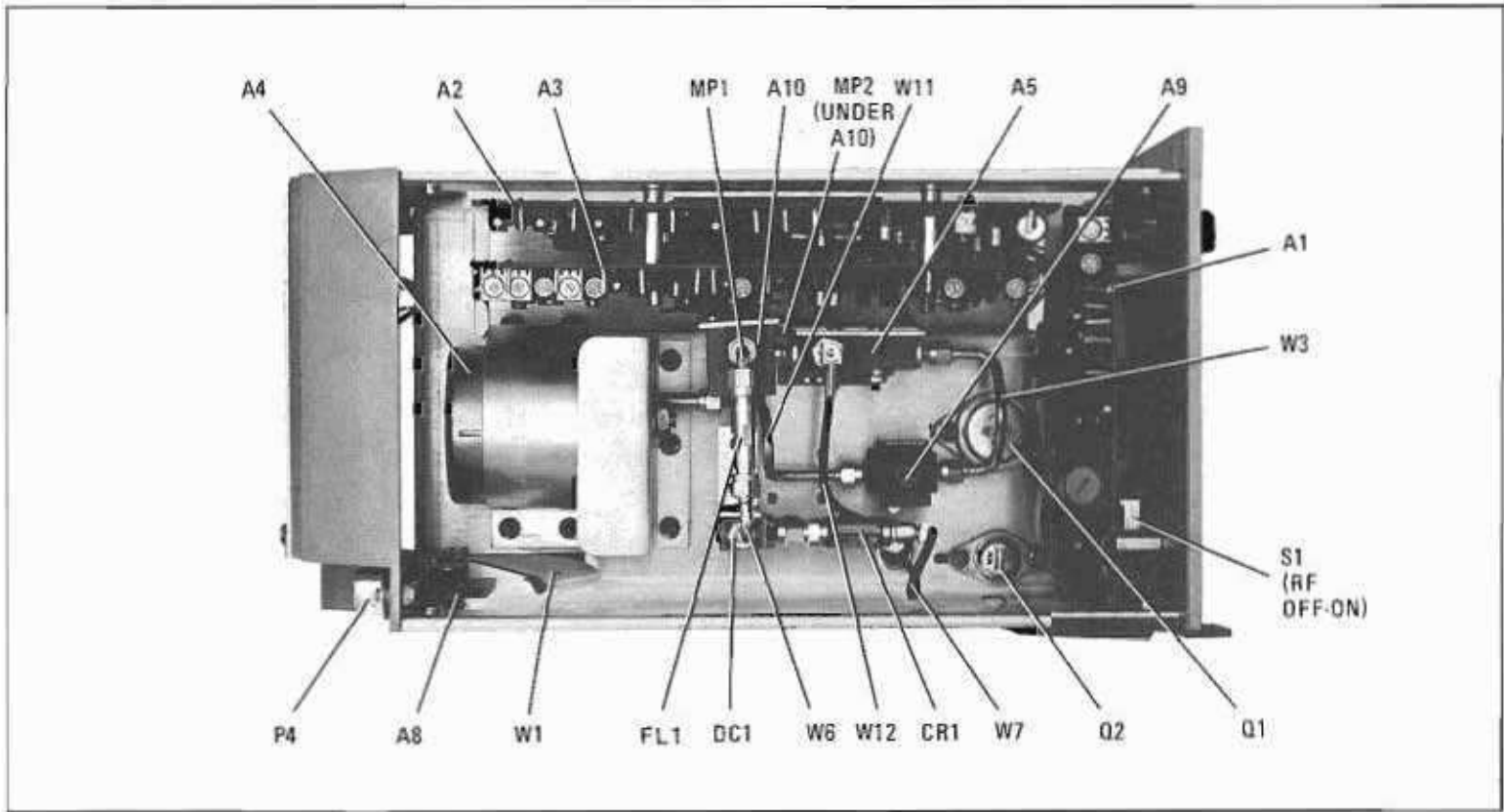
Figure 8-25. Major Assembly and Component Locations, Top View, 86242D/86250D (Option 001)
