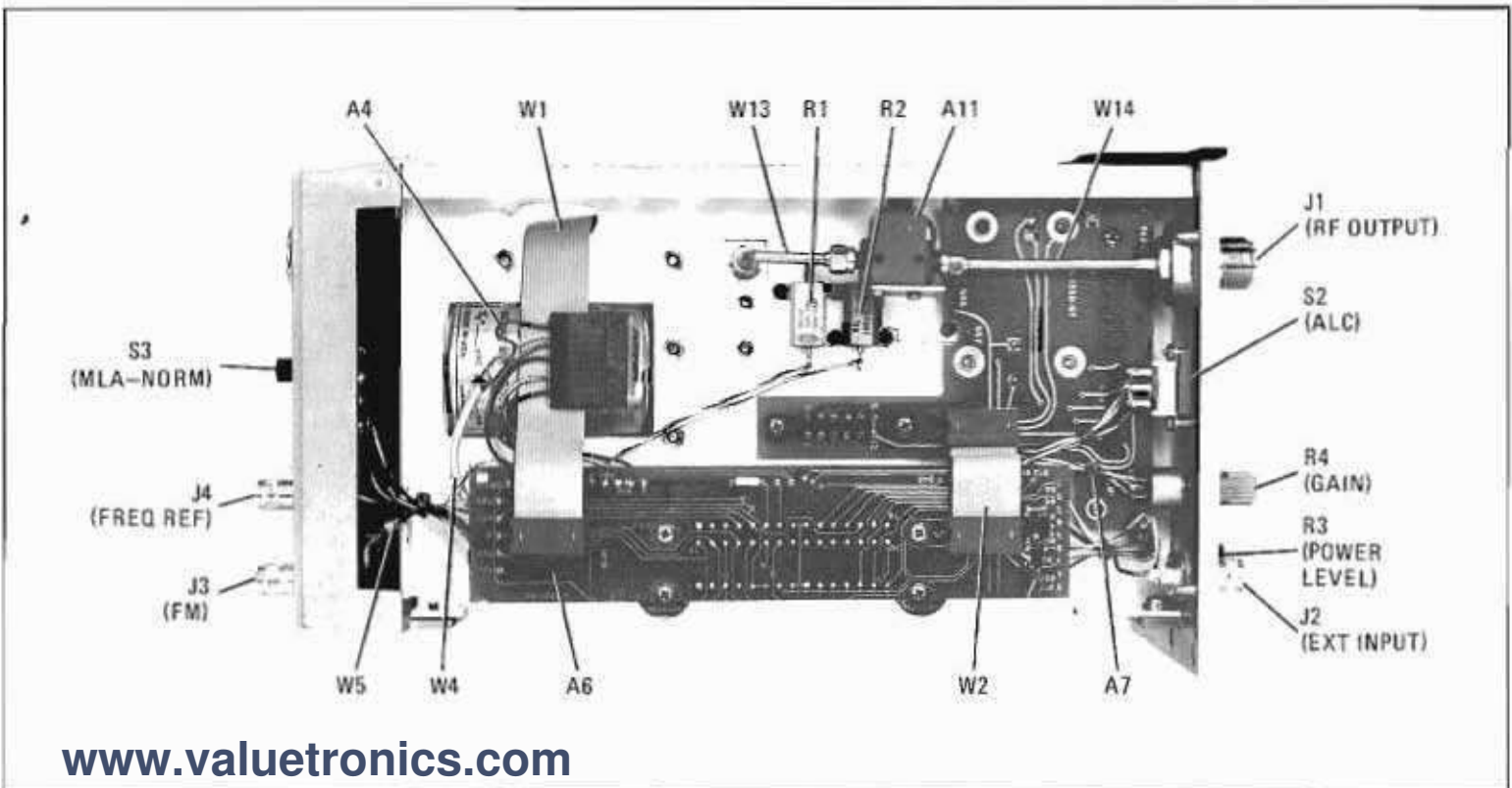
Figure 8-26. Major Assembly and Component Locations, Bottom View, 86242D/86250D (Option 008)
