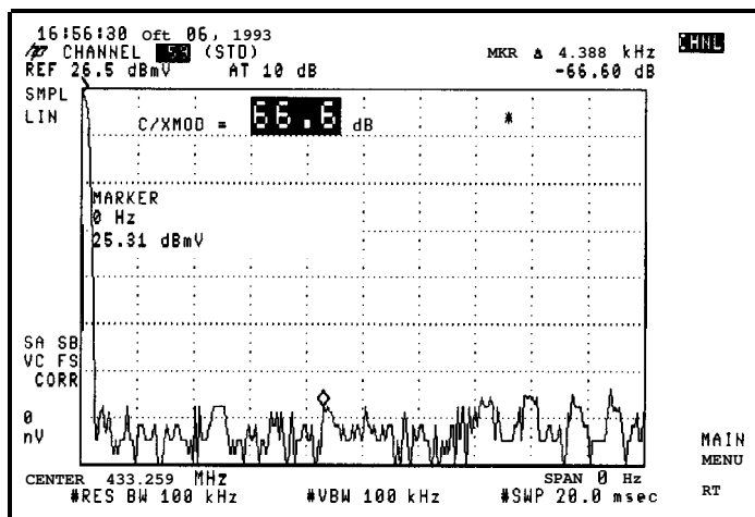
Figure 2-19. Cross Modulation Measurement
