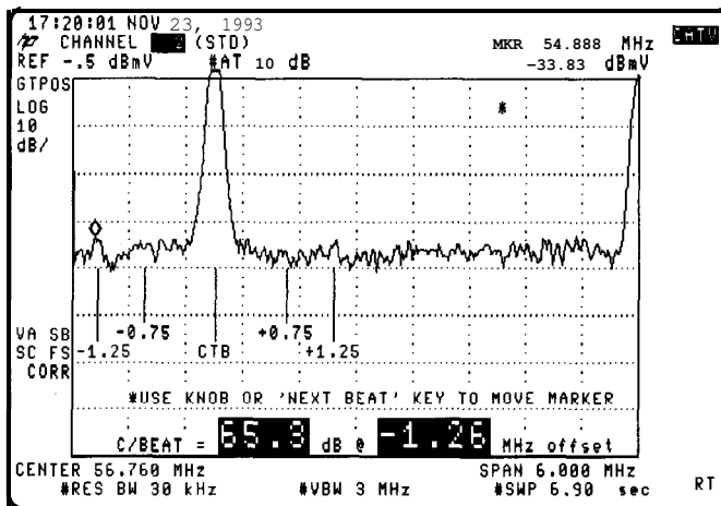
Figure 2-17. CSO Measurement
