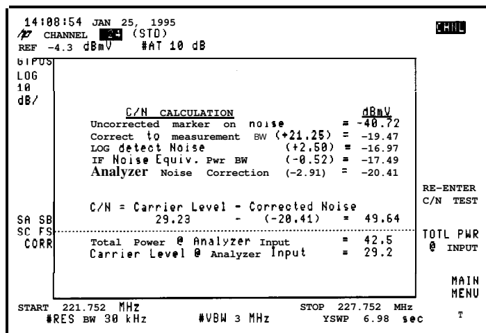
Figure 2-13. Carrier-to-Noise, More Information
