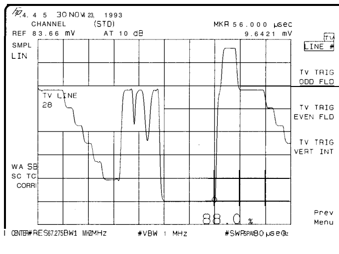
Figure 2-21. TV line Number
