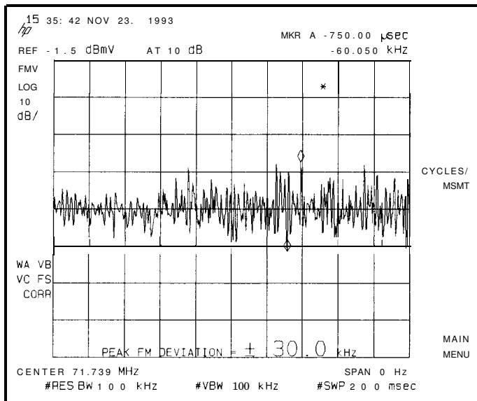
Figure 2-29. FM Deviation
