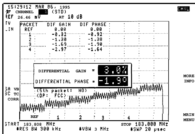
Figure 2-26. Differential Gain/Differential Phase, More Information
