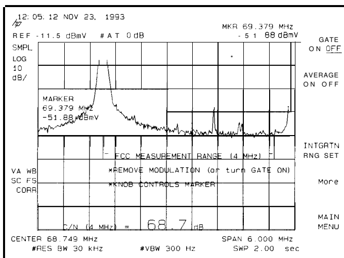
Figure 2-9. Carrier-to-Noise-Modulation and Gating Off
