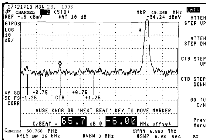
Figure 2-18. CTB Measurement
