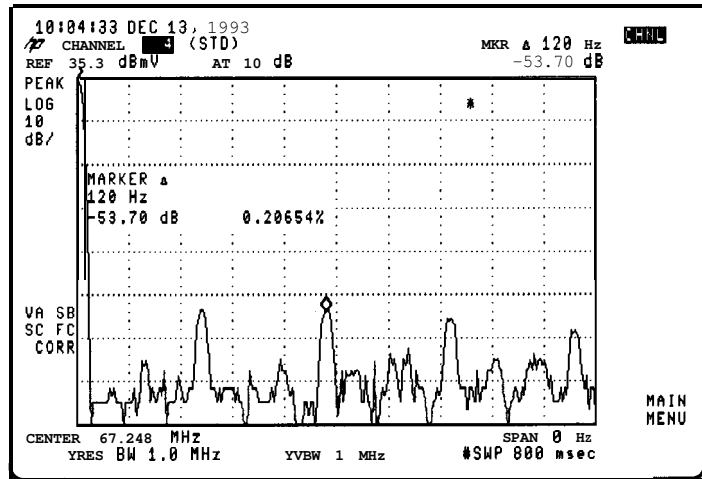
Figure 8-8. HUM, More Information
