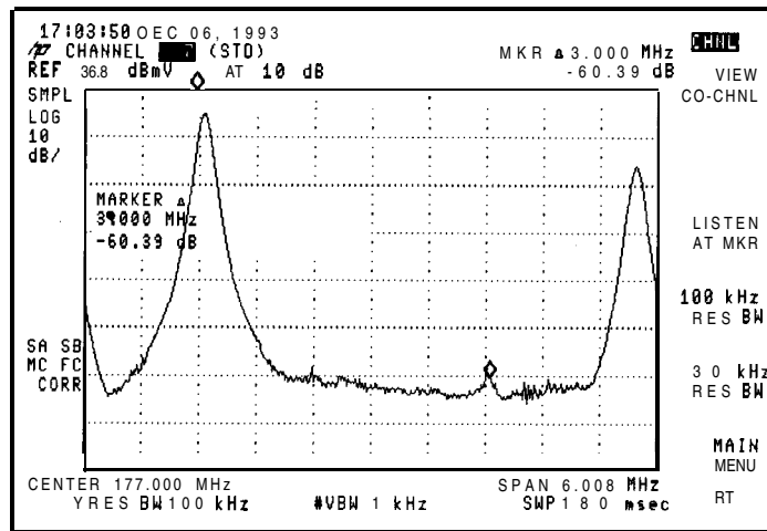
Figure 2-40. View Ingress
