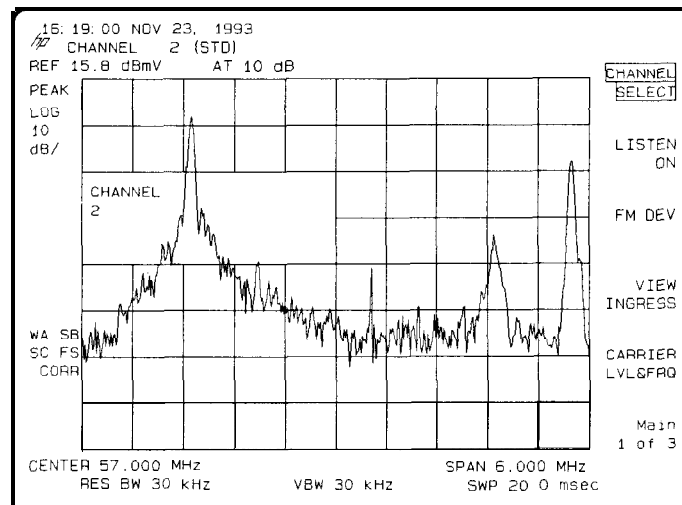
Figure 5-6. Channel Selected
