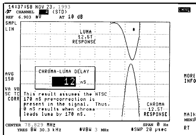
Figure 2-16. Chrominance to luminance, More Information
