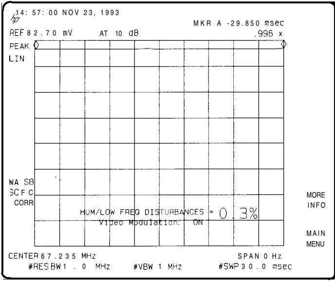
Figure 2-30. Hum Measurement
