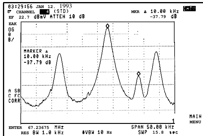
Figure 5-14. View Co-Channel
