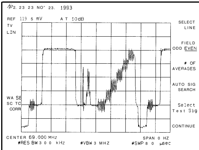
Figure 2-24. NTC 7 Composite Test Signal
