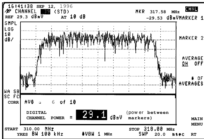
Figure 2-28. Results of Digital Channel Power Test
