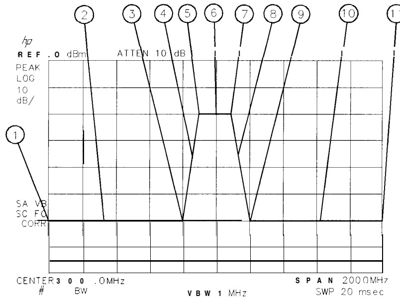
Figure 5-6. Limit-Line Segments
