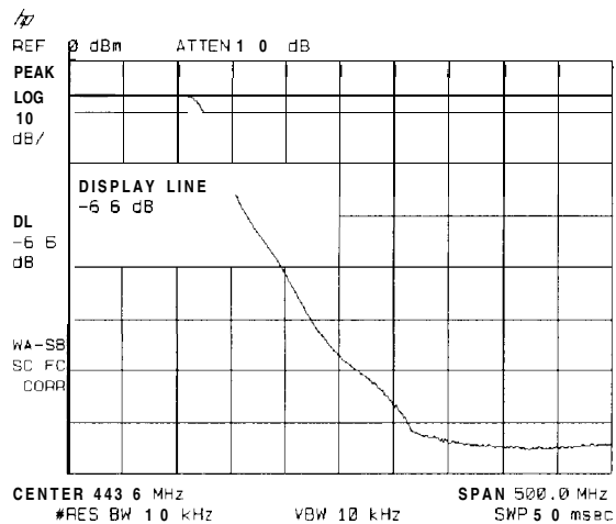
Figure 4-9. Normalized Trace
