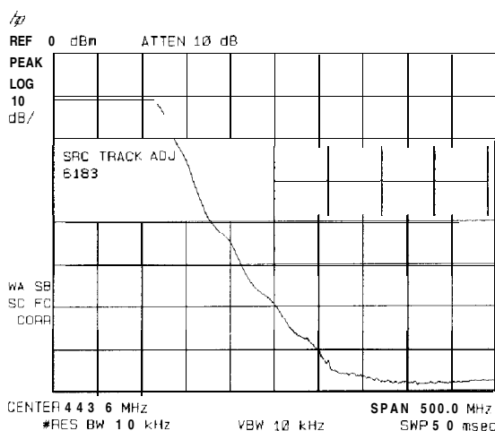
Figure 4-8. Manual Tracking Adjustment Compensates for Tracking Error
