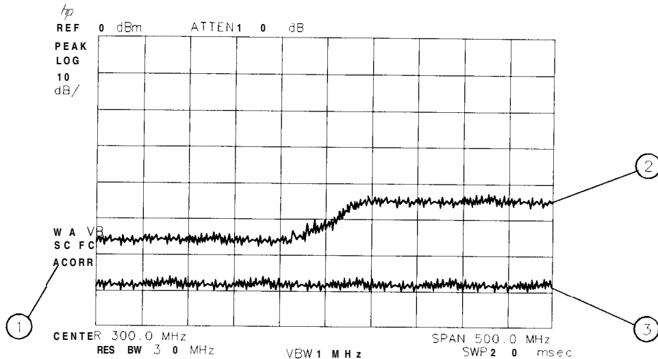
Figure 5-1 1. Amplitude-Correction Display
