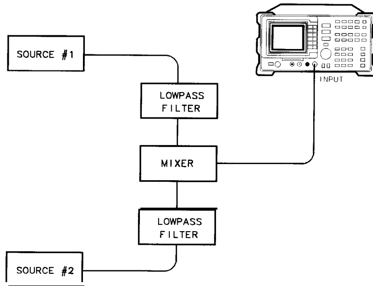
Figure 3-24. Third-Order Intermodulation Equipment Setup
