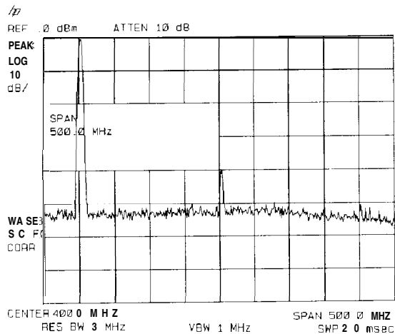
Figure 3-21. Harmonic Distortion
