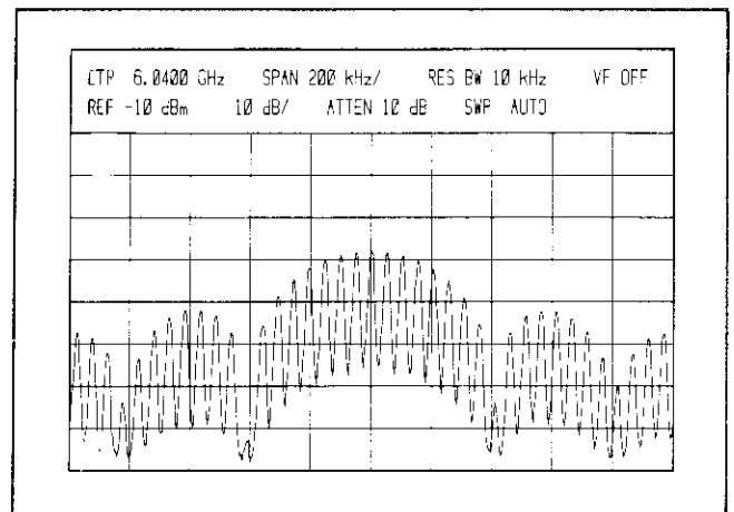
Figure 41. Line Spectrum
