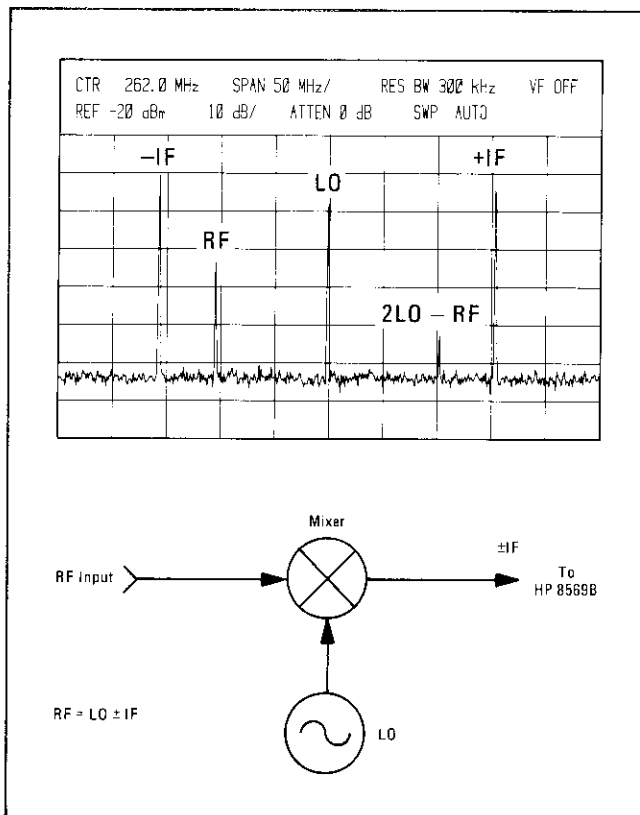
Figure 33. Mixer Measurement
