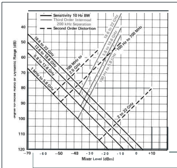
Fig. 4. Typical optimum dynamic range
