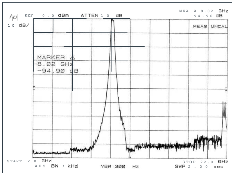
High dynamic range scalar measurement
