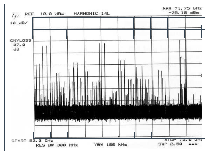
Harmonic mixing extends frequency range.
