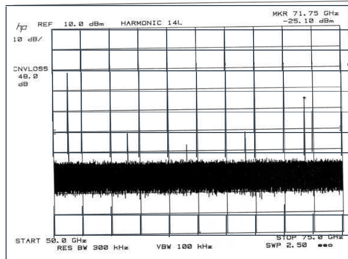
Preselected mixers eliminate images and multiples.
