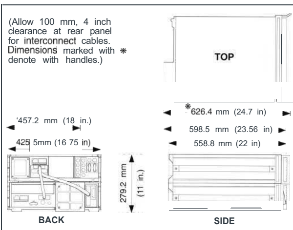
Fig.7. Instrument dimensions with and without handles
