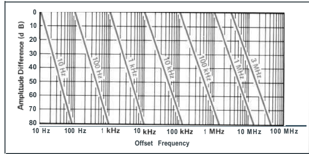
Fig. 1. Typical spectrum analyzer resolution
