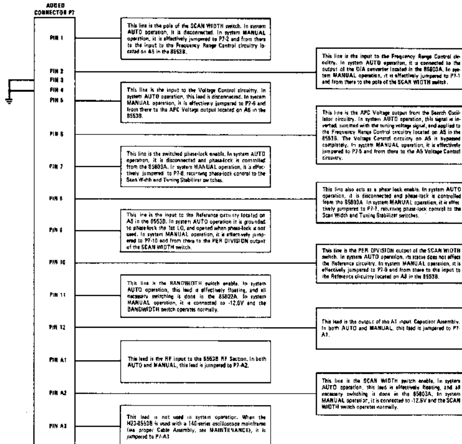
Figure 1. Connections to Added Connector P7
