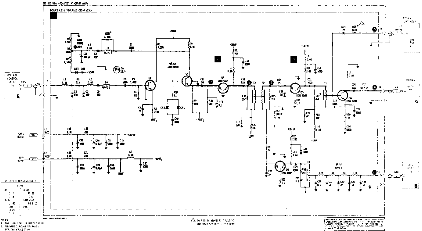
Figure B-33. 206.361 MHz Voltage Tuned Oscillator (ERRATA)
