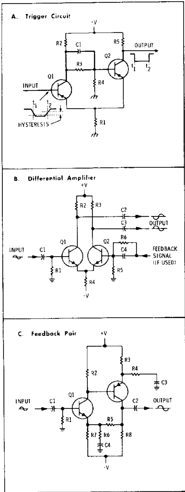
Figure 8-5. Basic Transistor Circuits.
