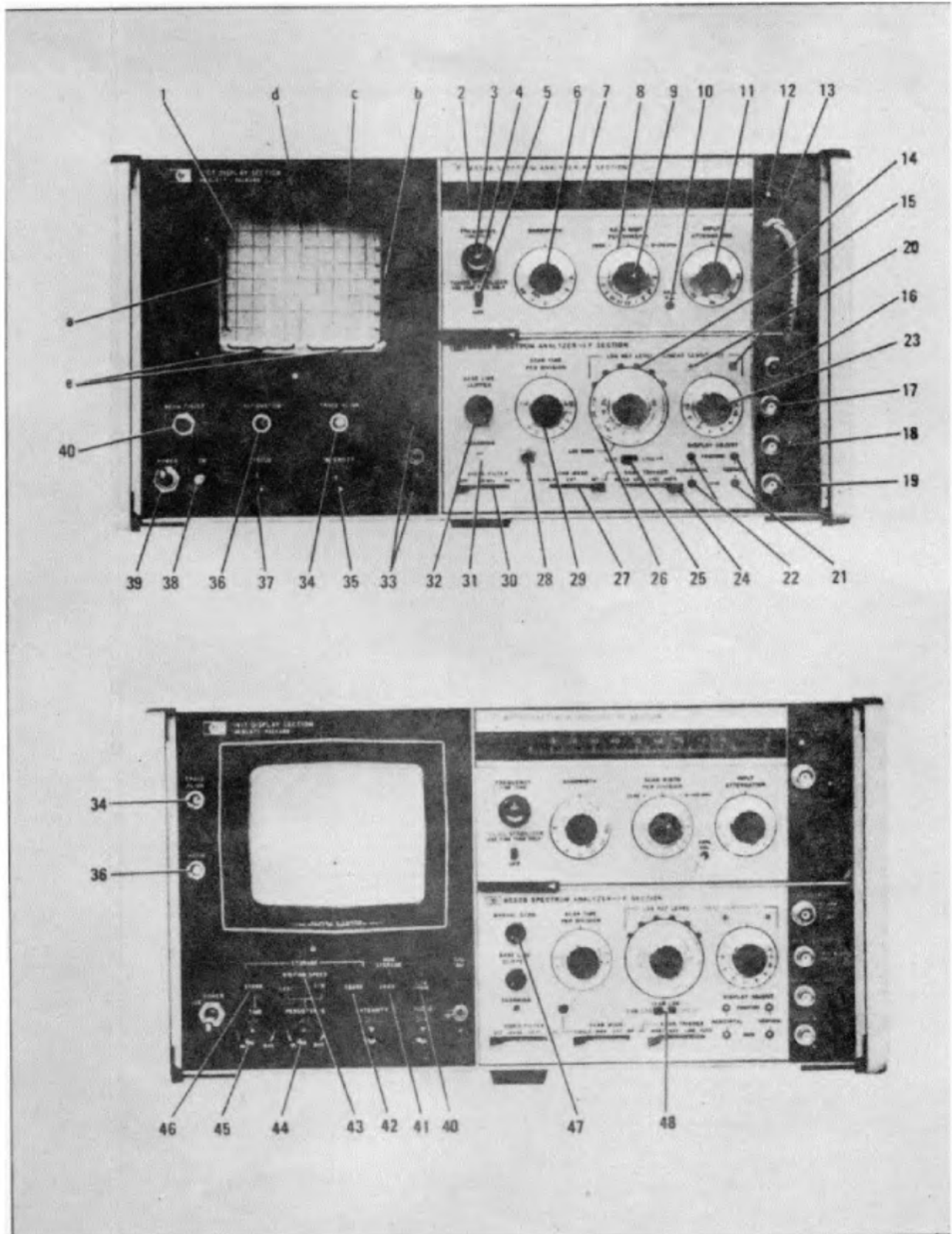
Figure 3-1. Spectrum Analyzer Controls, Indicators and Connectors (cont'd)
