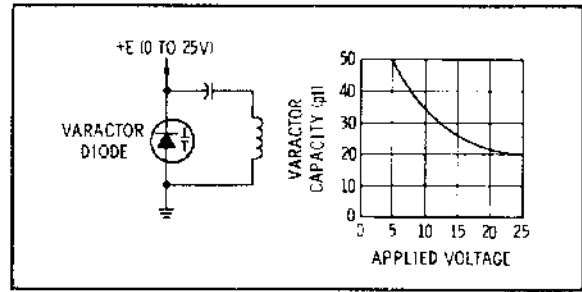
Figure 8-12. Varactor Characteristics.
