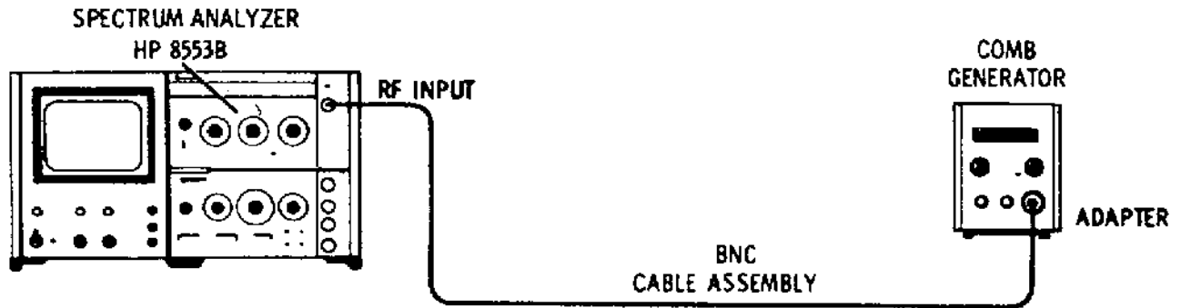
Figure 4-5. Scan Width Accuracy Test: 10 MHz/Div
