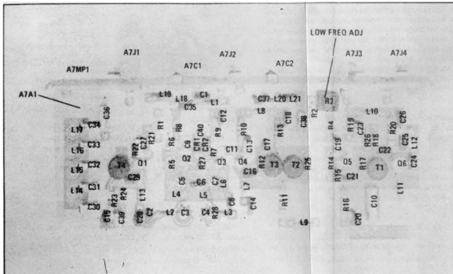
Figure 8-32. 200-310 MHz VTO Assembly A7 (08553-6003) Component Locations
