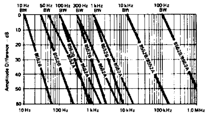
Figure 1-3. Typical Resolution
