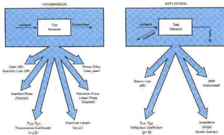
Basic B505A Transmission and Reflection Measurements
