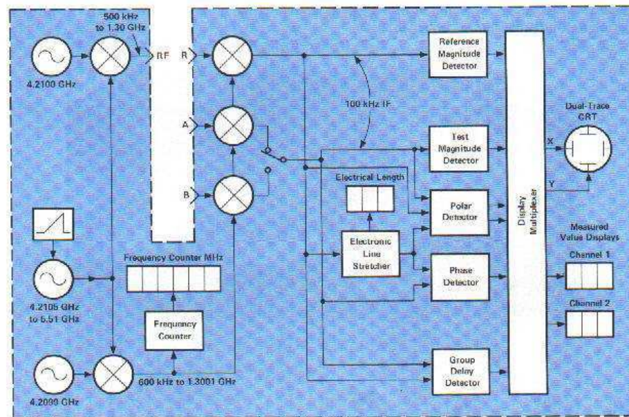
B505A Simplified Block Diagram
