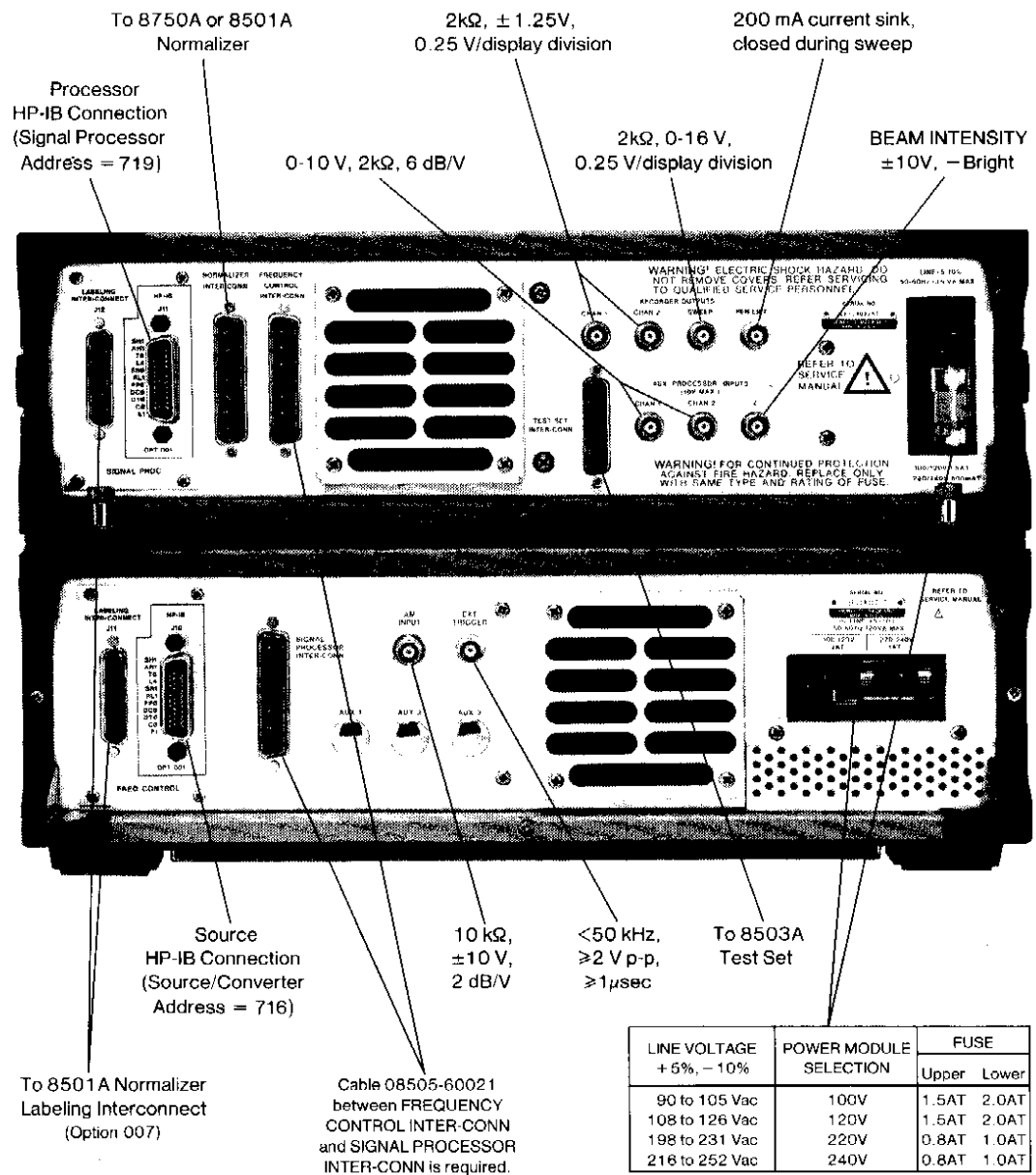
8505A Rear Panel Connections
