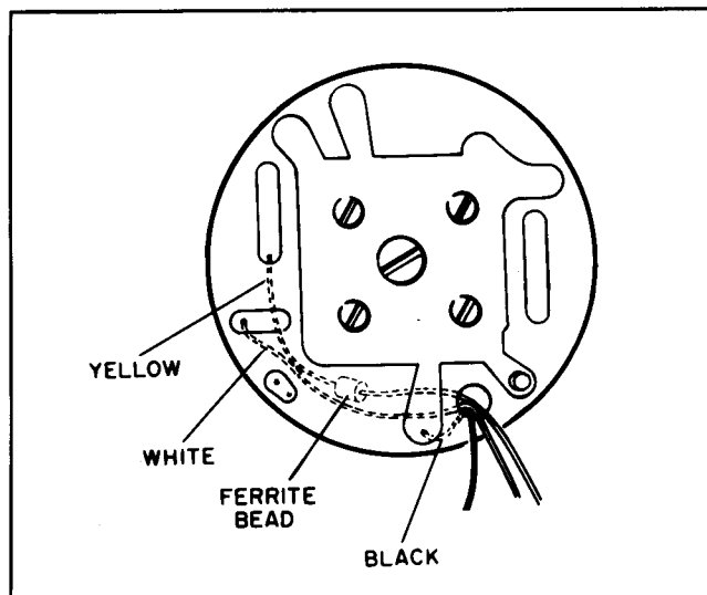
Figure A8. Printed Circuit Board (P/O Change C)
