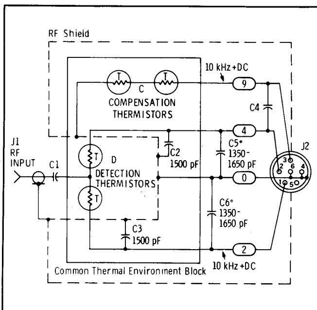
Figure A2. 8478B Connected to a 431C Power Meter (P/O Change A)
