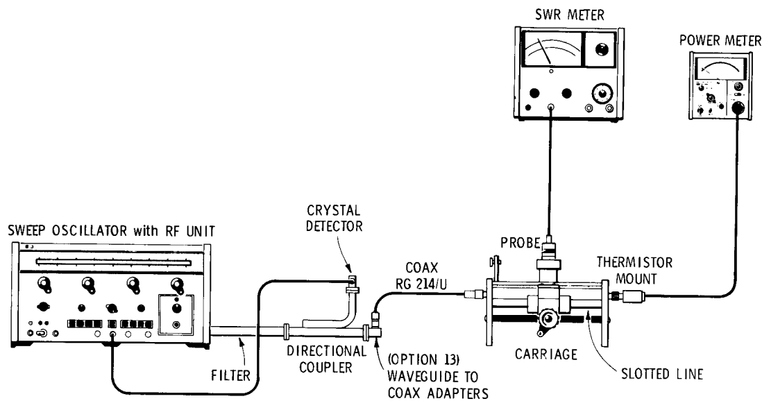
Figure 7. SWR Measurement, 15 and 18 GHz
