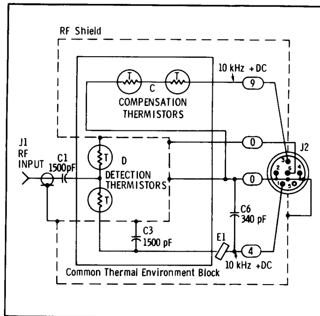
Figure 5. 8478B Connected to a 431C Power Meter
