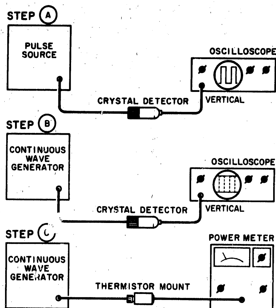
Figure 1. Peak Power Measurement
