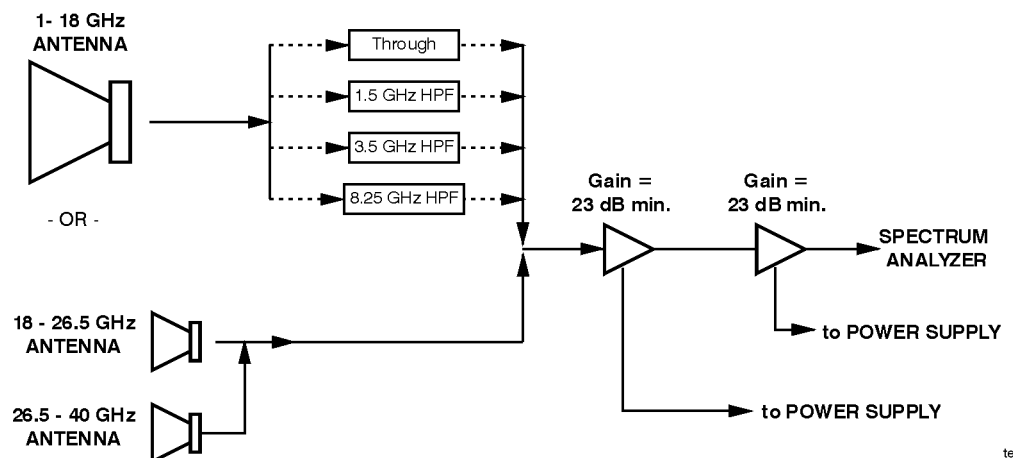
Figure 4-1. Test Set Diagram
