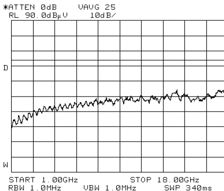
Figure 2-2. Typical Sensitivity from 1 to 18 GHz
