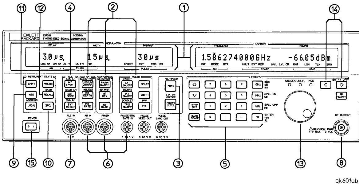
HP 83731B/32B Synthesized Signal Generator
