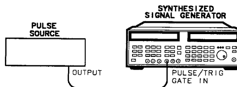
Figure 3-8. Doublet Pulse Equipment Setup
