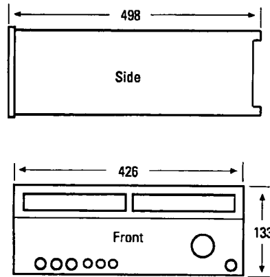
Figure 4-10. Dimensions
