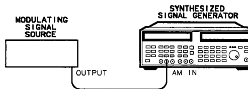
Figure 3-15. External Linear AM Equipment Setup
