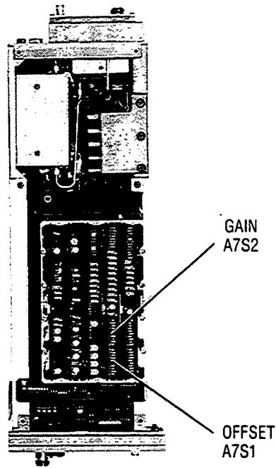
Figure 5-18. SYTM to YO Tracking Calibration Switch Location
