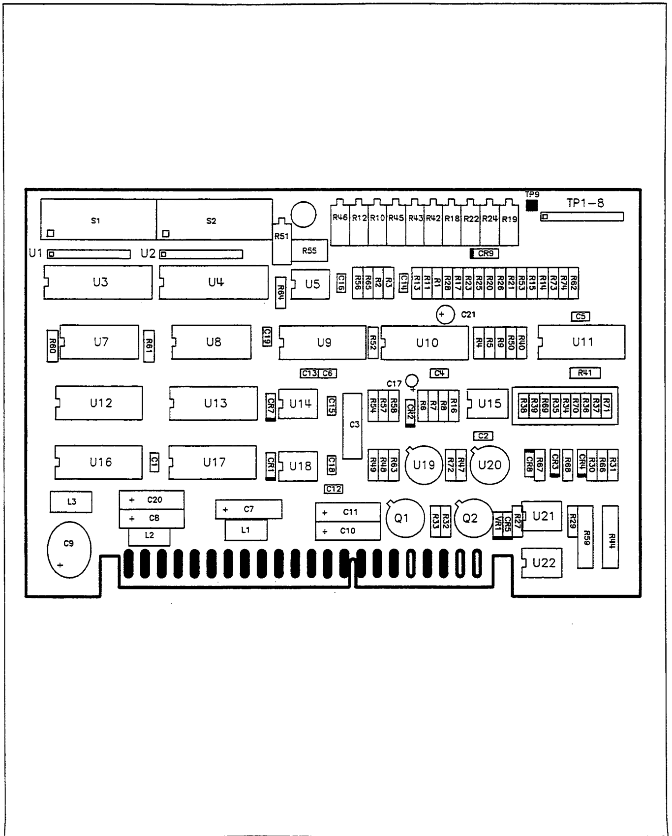
Figure 8-58. A7 SYTM Driver Components Location Diagram
