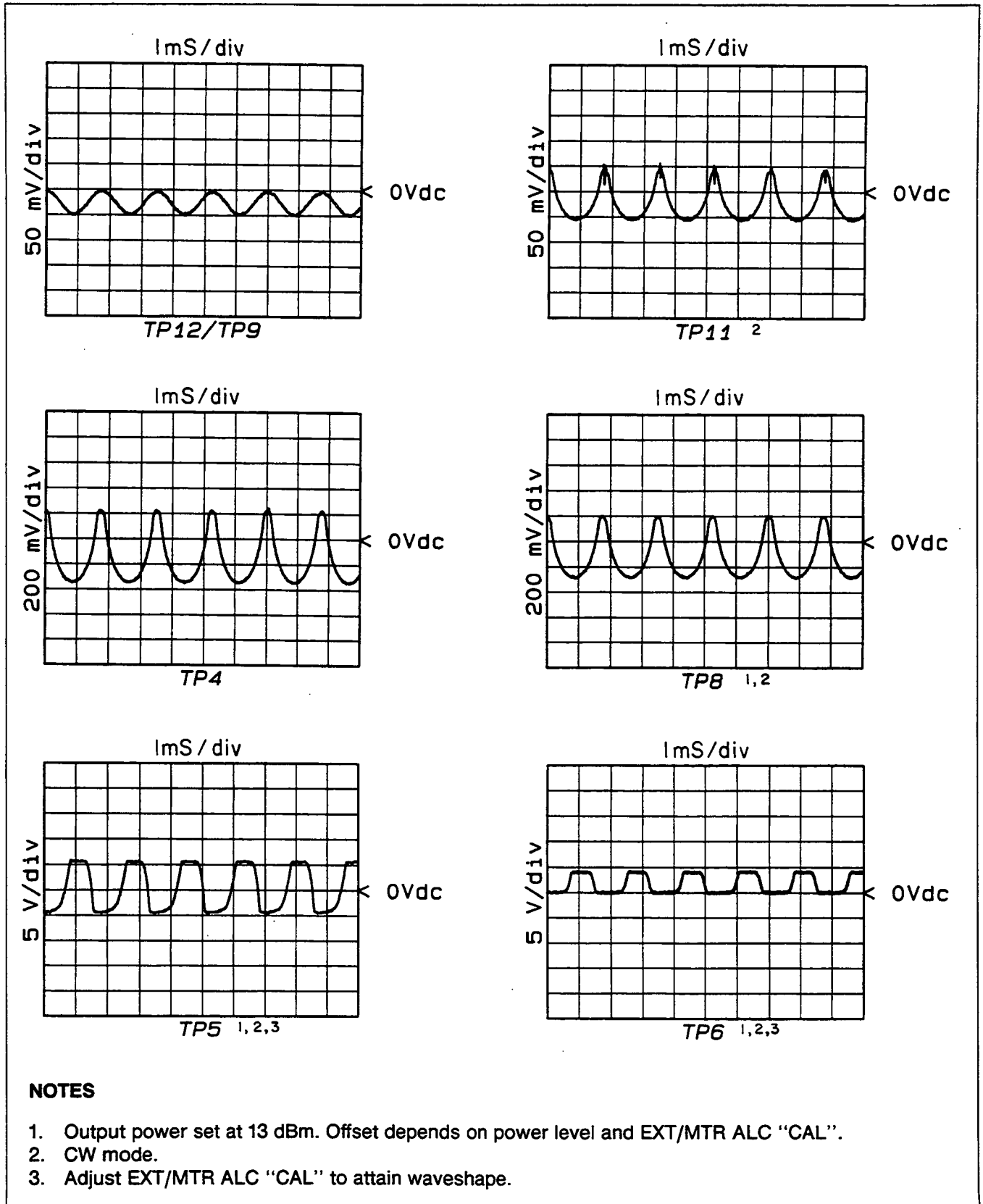
Figure 8-29. Open Loop Waveforms
