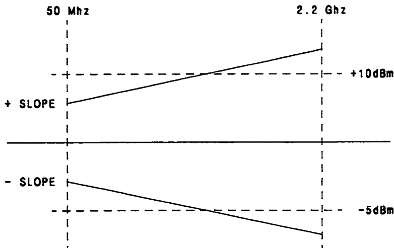
Figure 5-32. 0 Slope Adjustment
