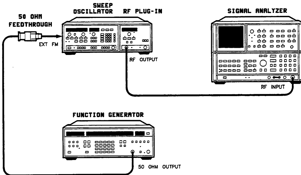
Figure 4-8. 100 Hz External Frequency Modulation Test Setup
